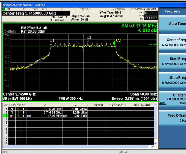
11AC20SISO-Ant2-5745-PASS
