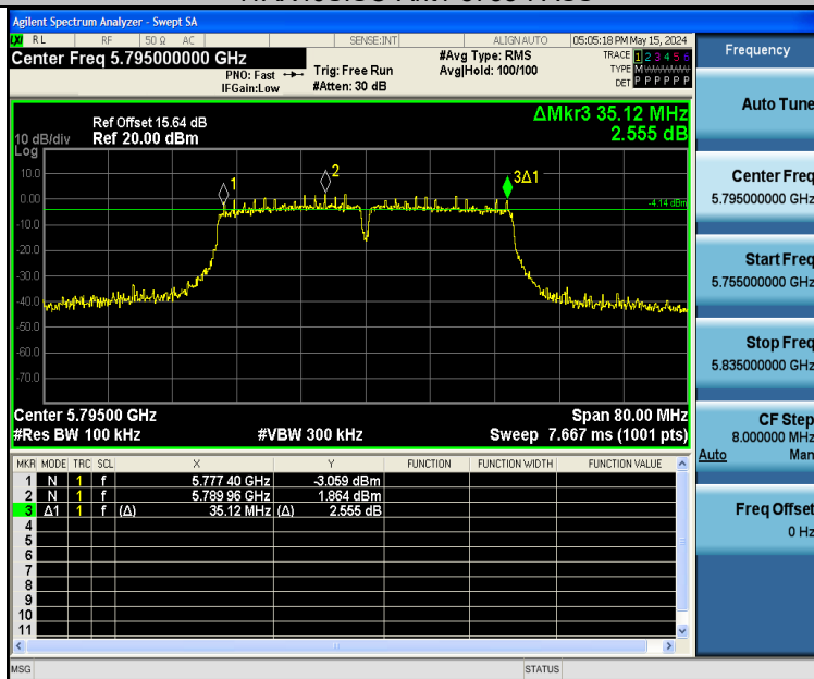
11AX40SISO-Ant1-5795-PASS
