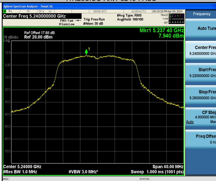
11N20SISO-Ant2-5240-PASS
