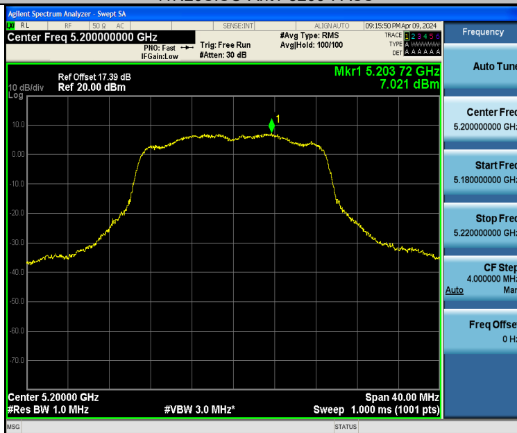
11N20SISO-Ant2-5200-PASS
