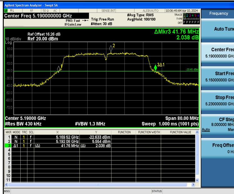
11AC40SISO-Ant2-5190
