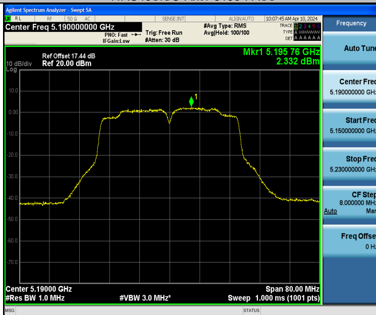
11AC40SISO-Ant2-5190-PASS
