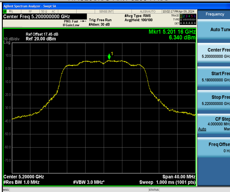
11AC20SISO-Ant2-5200-PASS
