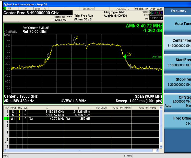
11AX40SISO-Ant1-5190
