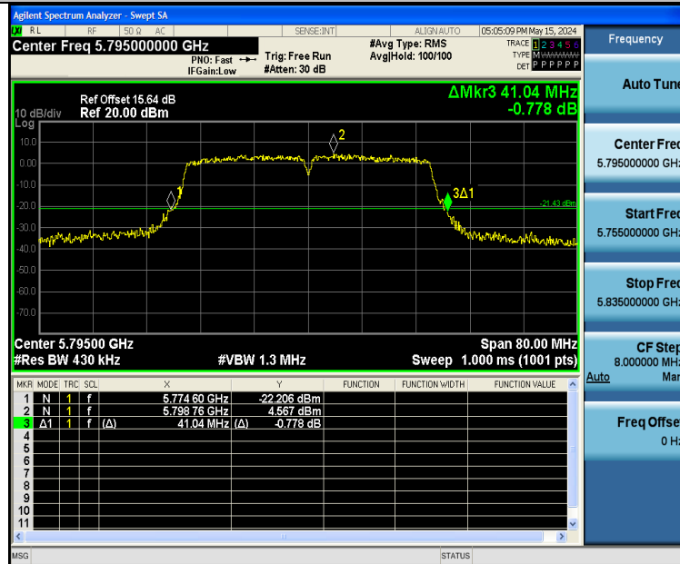
11AX40SISO-Ant1-5795
