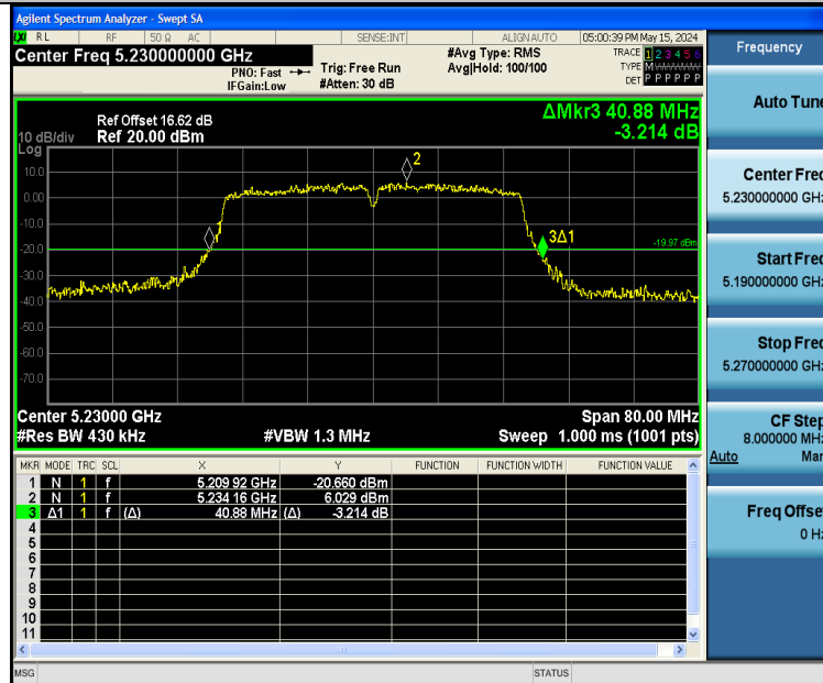
11AX40SISO-Ant1-5230
