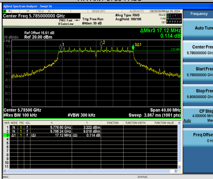
11A-Ant2-5785-PASS
