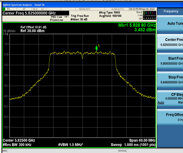
11N20SISO-Ant2-5825-PASS
