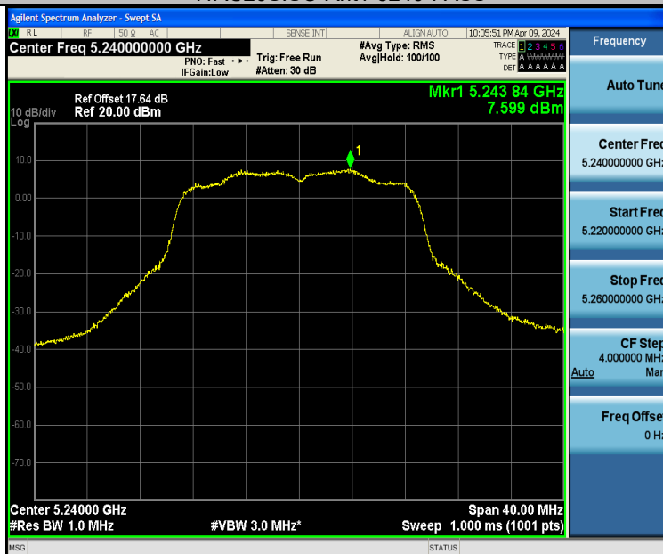
11AC20SISO-Ant2-5240-PASS
