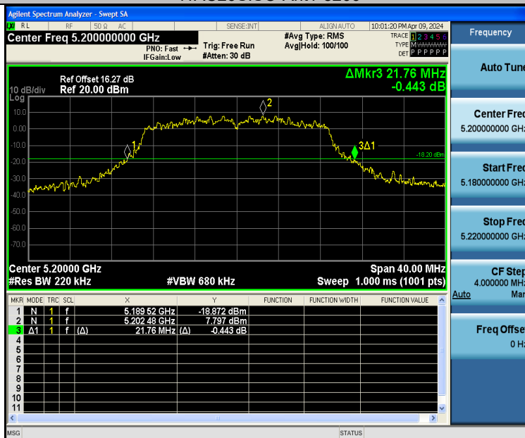
11AC20SISO-Ant2-5200
