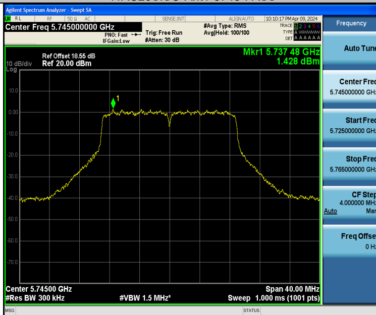
11AC20SISO-Ant2-5745-PASS
