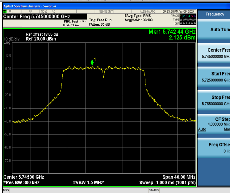
11N20SISO-Ant2-5745-PASS
