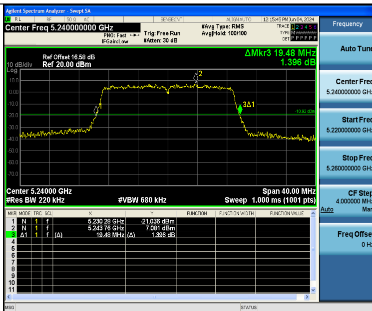
11AX20SISO-Ant2-5240
