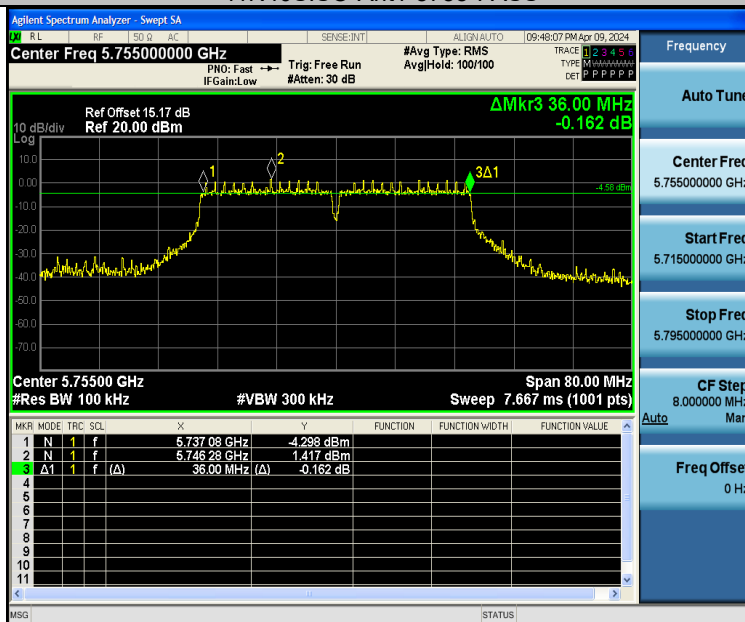
11N40SISO-Ant2-5755-PASS
