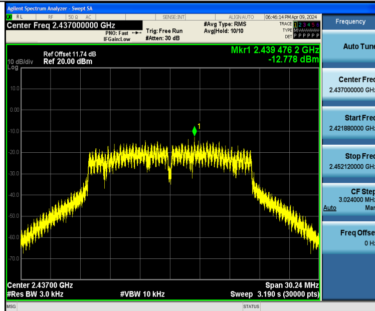
11G-Ant2-2437-PASS
