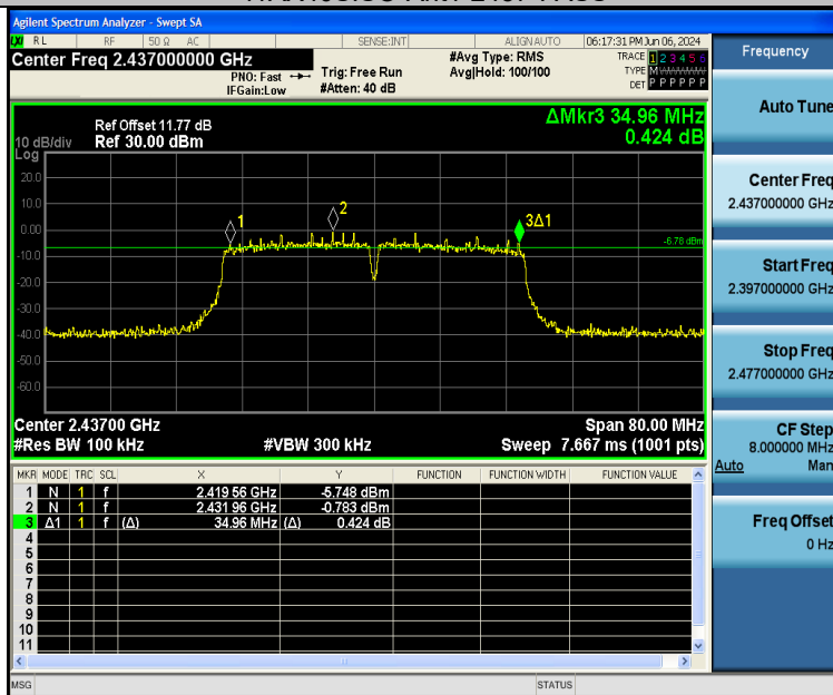
11AX40SISO-Ant2-2437-PASS
