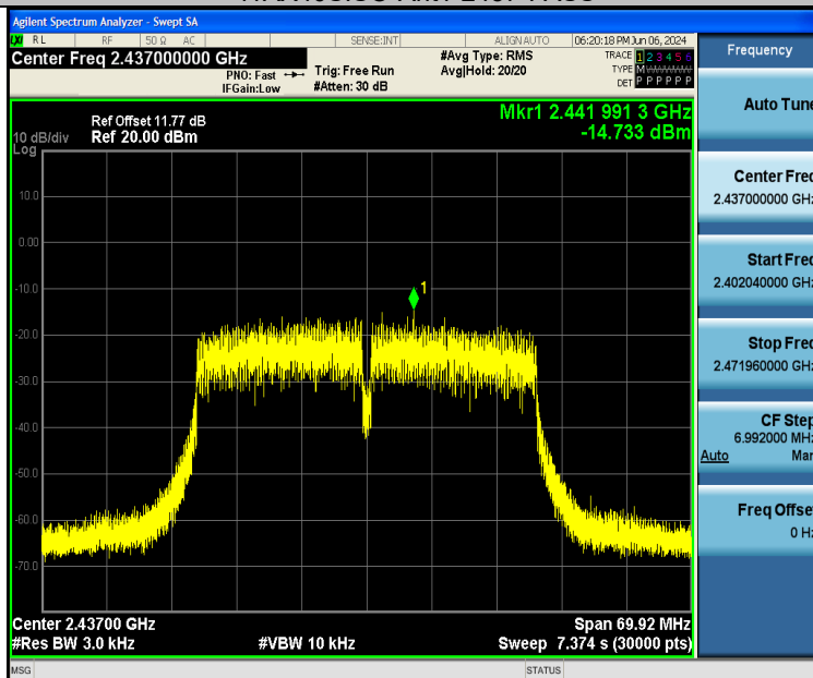
11AX40SISO-Ant2-2437-PASS
