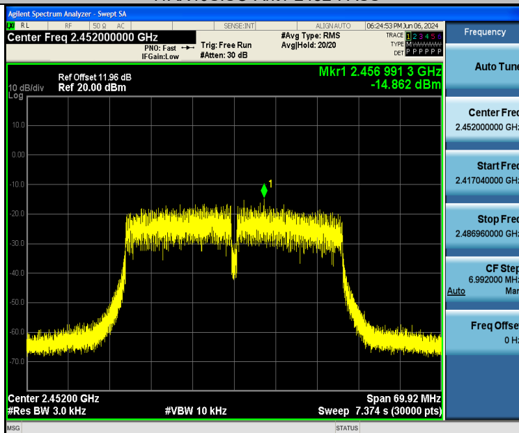
11AX40SISO-Ant2-2452-PASS
