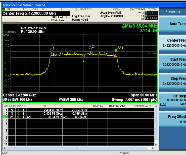
11AX40SISO-Ant2-2422-PASS
