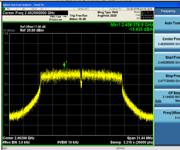
11AX20SISO-Ant2-2462-PASS
