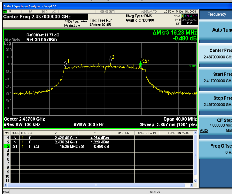
11AX20SISO-Ant2-2437-PASS
