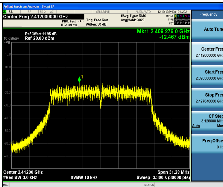
11AX20SISO-Ant1-2412-PASS
