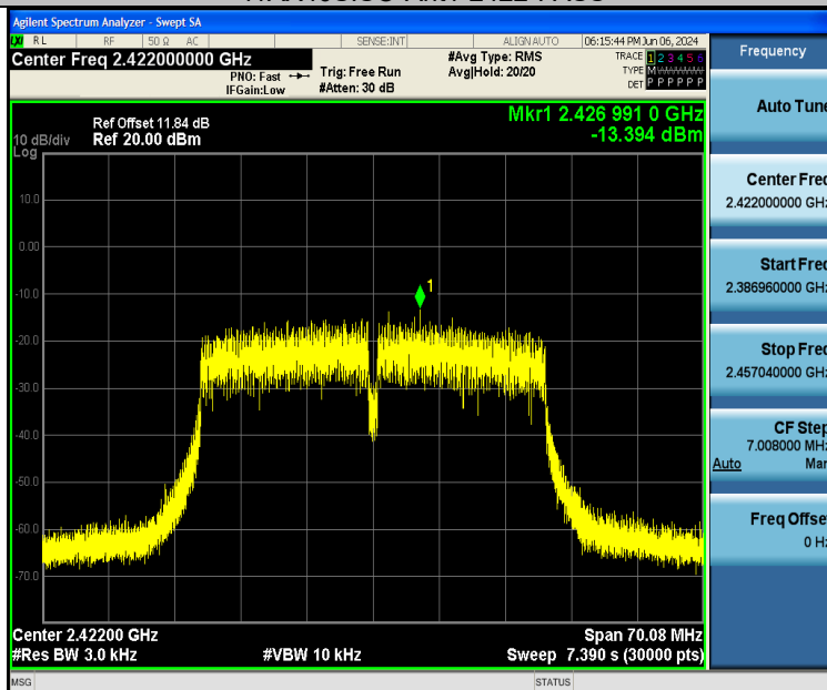
11AX40SISO-Ant2-2422-PASS
