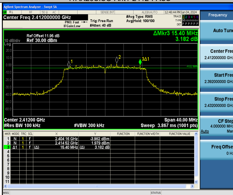
11AX20SISO-Ant2-2412-PASS
