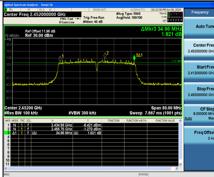
11AX40SISO-Ant2-2452-PASS
