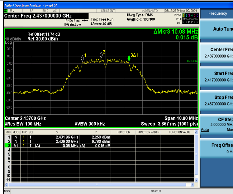
11B-Ant2-2437-PASS
