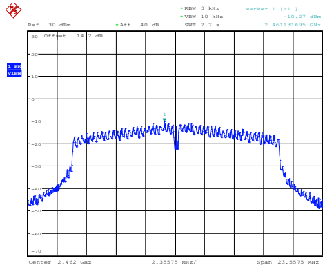
IEEE 802.11g High CH Chain0
