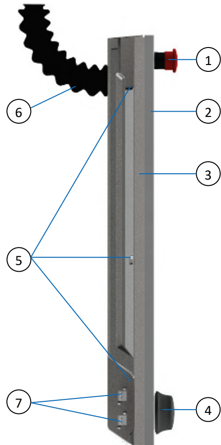
Fig. 22: Left side of the CC300 operator panel
