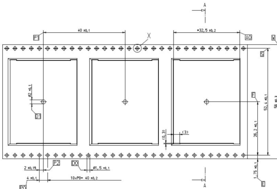
Figure 41: Feed direction
