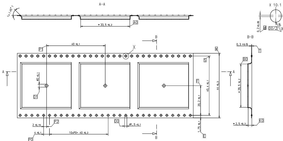
Figure 51: Carrier tape
