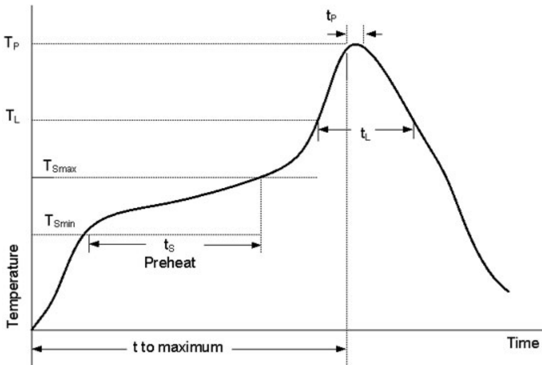
Figure 51: Reflow Profile
