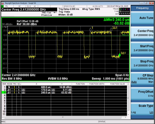
NTNV-11G-Ant1-2412
