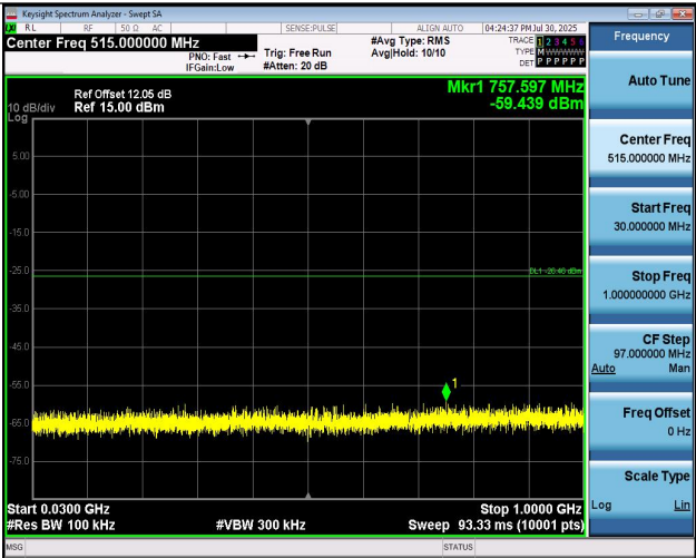
11AX20SISO-Ant1-2412-30~1000-PASS
