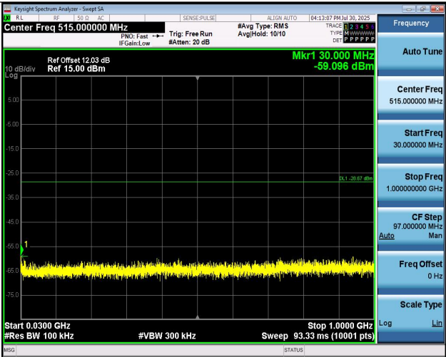
11N40SISO-Ant1-2422-30~1000-PASS
