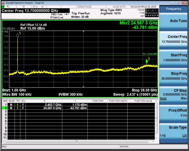
11N40SISO-Ant1-2452-1000~26500-PASS
