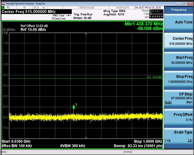
11N40SISO-Ant1-2437-30~1000-PASS
