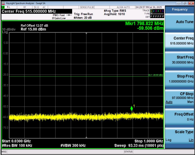
11AX20SISO-Ant1-2462-30~1000-PASS
