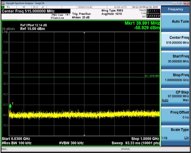
11N40SISO-Ant1-2452-30~1000-PASS
