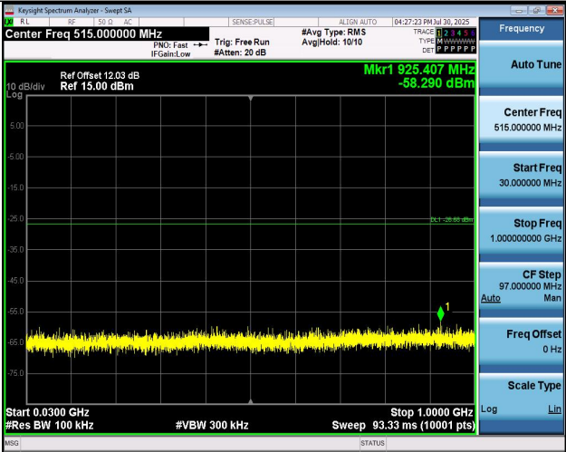
11AX20SISO-Ant1-2437-30~1000-PASS
