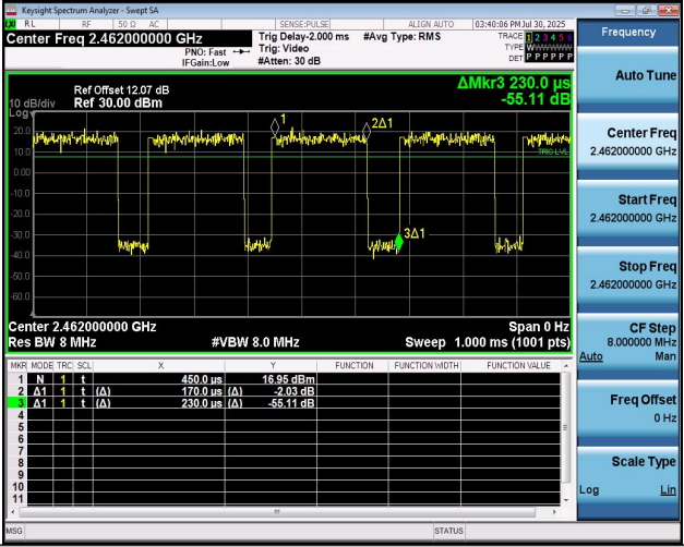
NTNV-11G-Ant1-2462
