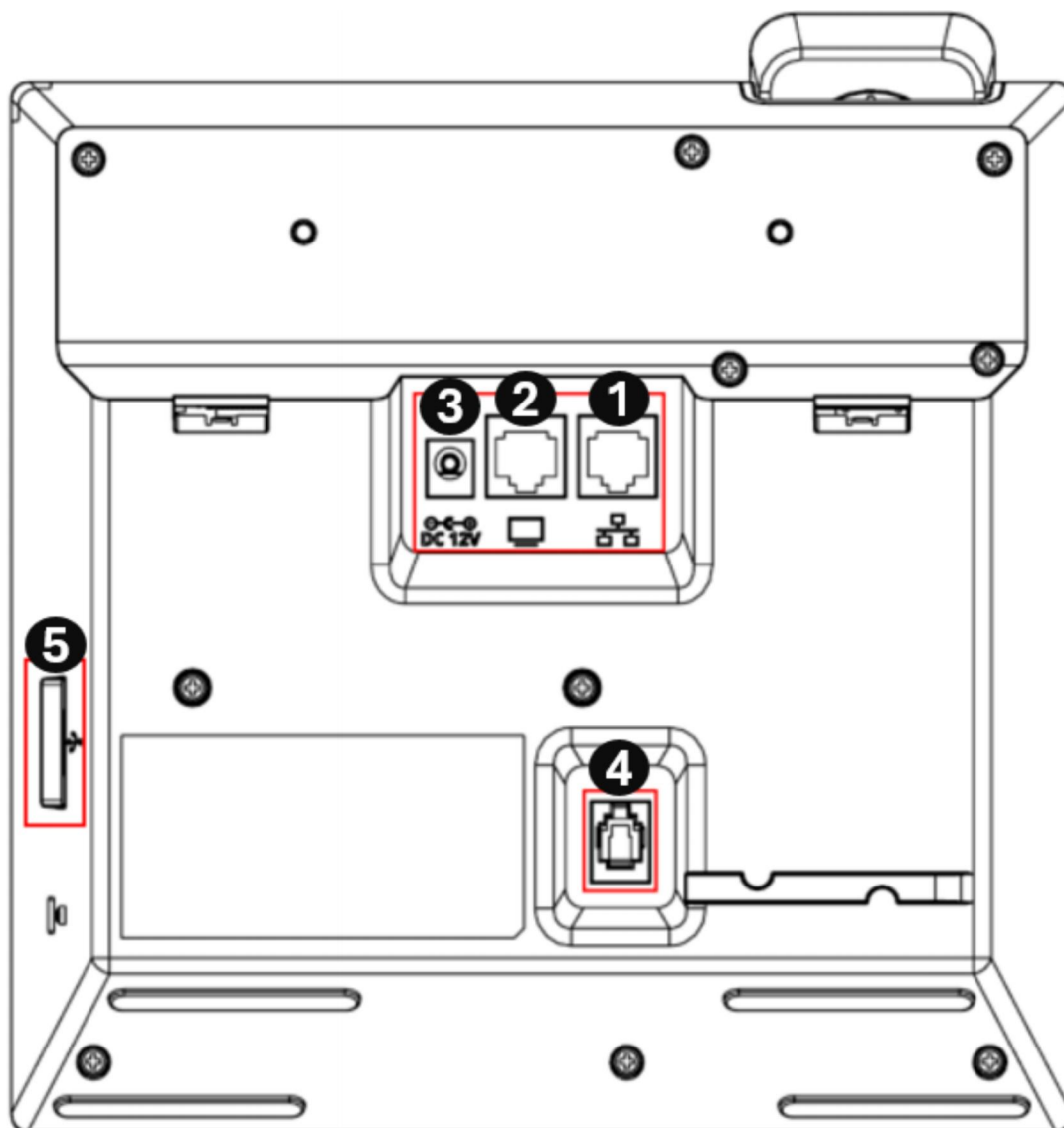
Figure 2-2: Rear View
