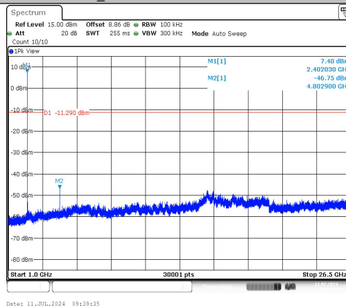
BLE_1M-Ant1-2402-1000~26500-PASS
