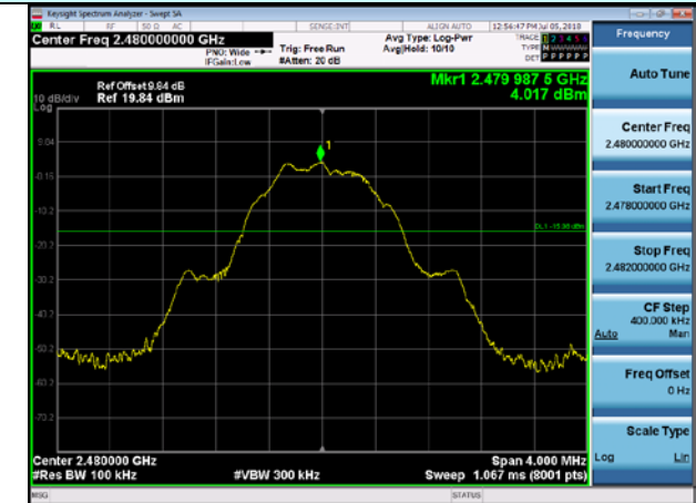
Bandedge Emission- Highest channel
