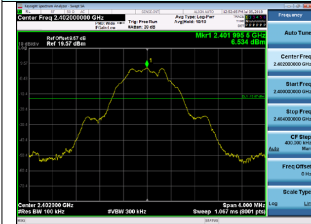
Bandedge Emission- Lowest channel
