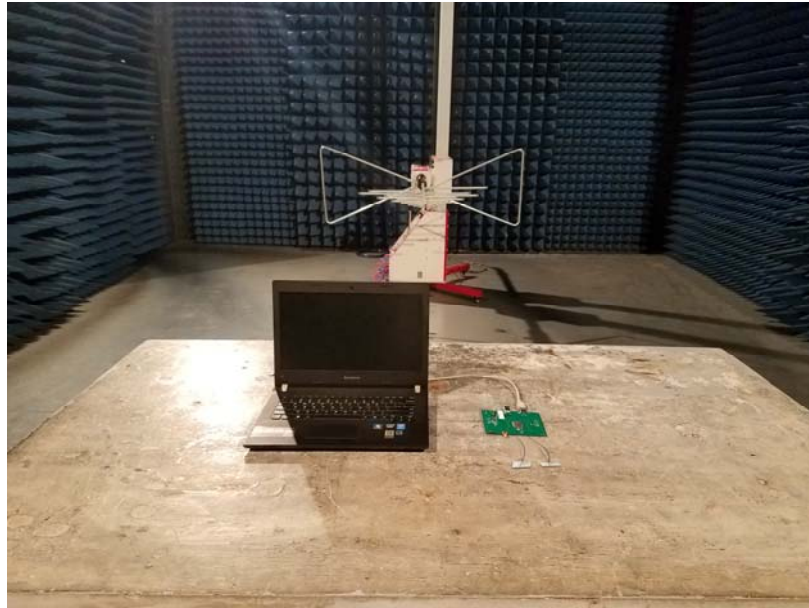
Model No.: 6222D-UUB Radiated Emission
