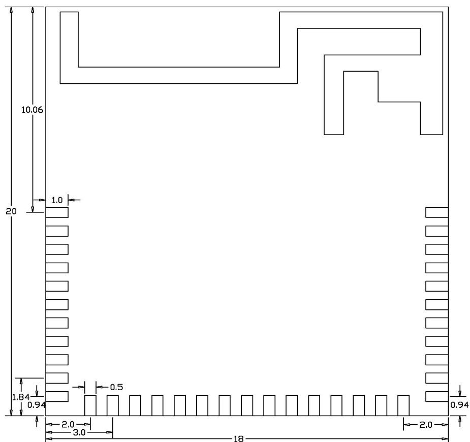
<TOP View>
