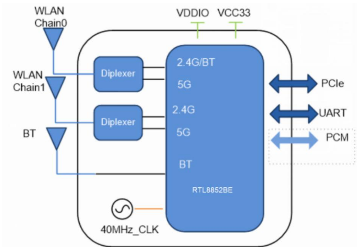
3 ANT version
