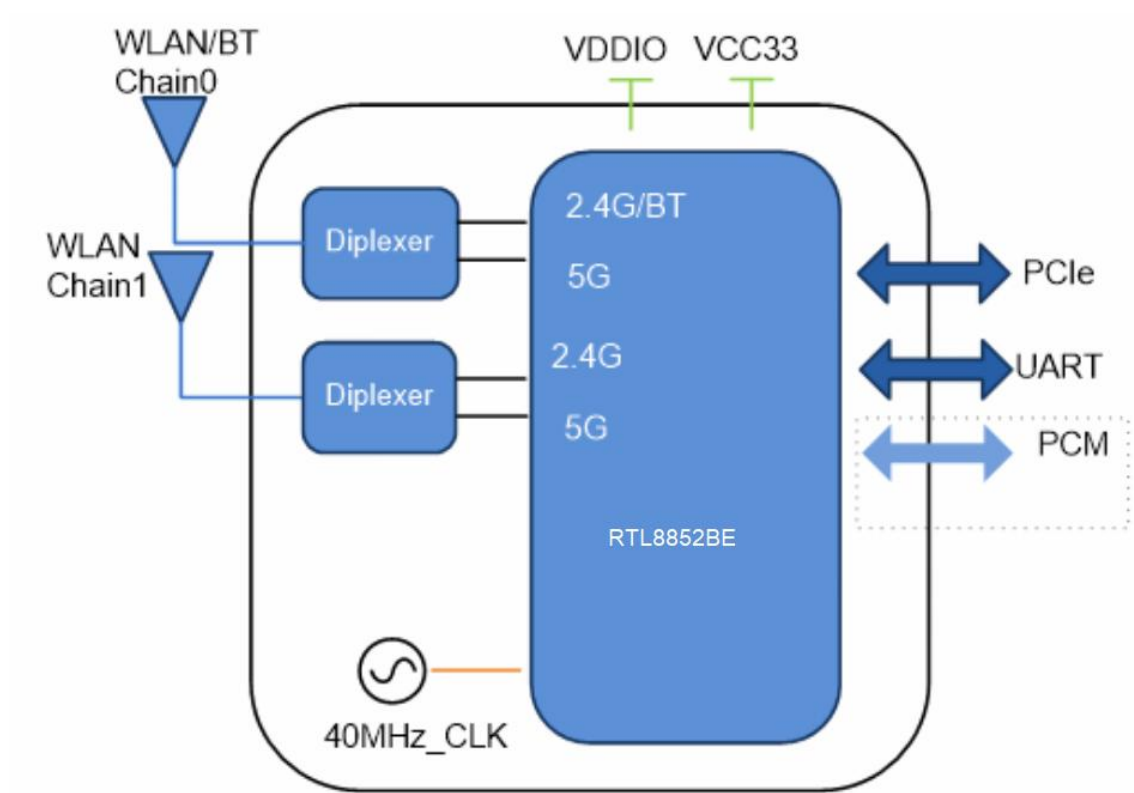
2 ANT version
