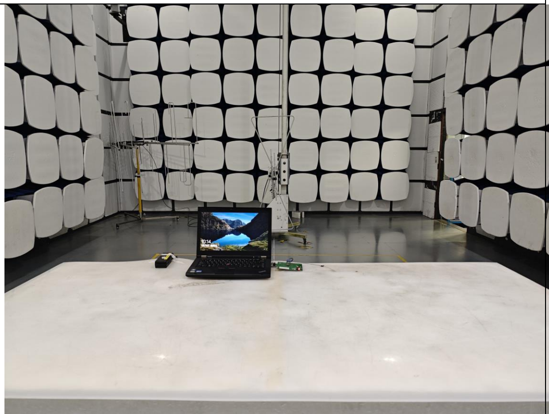
Radiated Emission
