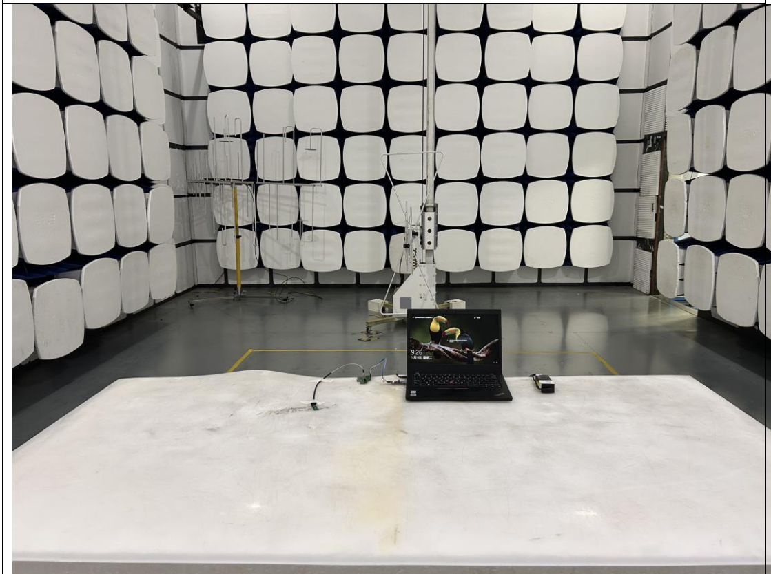
Radiated Emission
