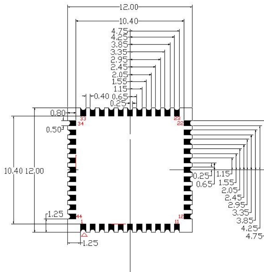
<TOP View>
