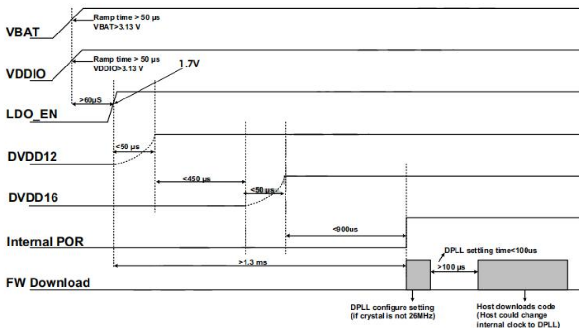
Figure 4 : Power-on sequence
