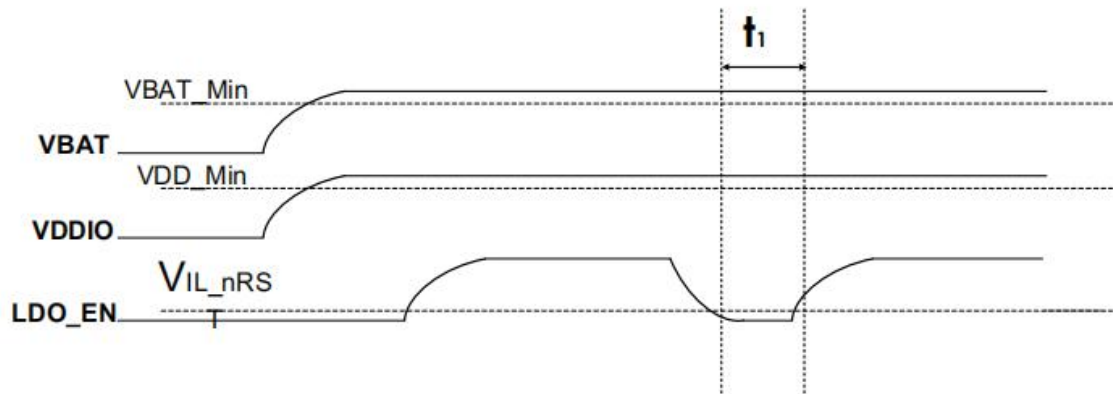
Figure 5 : Reset Timing
