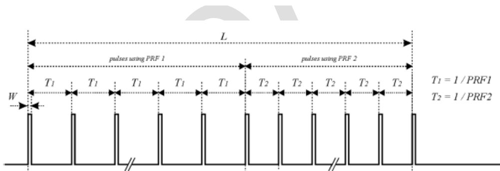
Figure D.4: General structure of a single burst/packet based staggered PRF radar test signal
