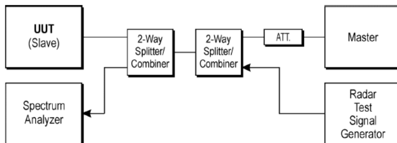
Figure 7: Set-up C
