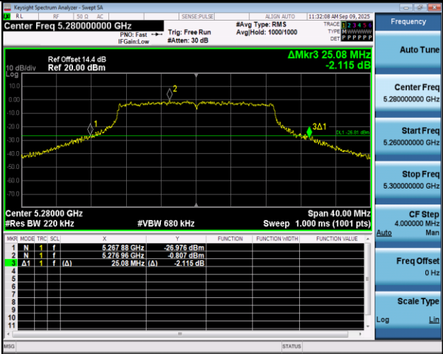
11N20SISO-Ant1-5280
