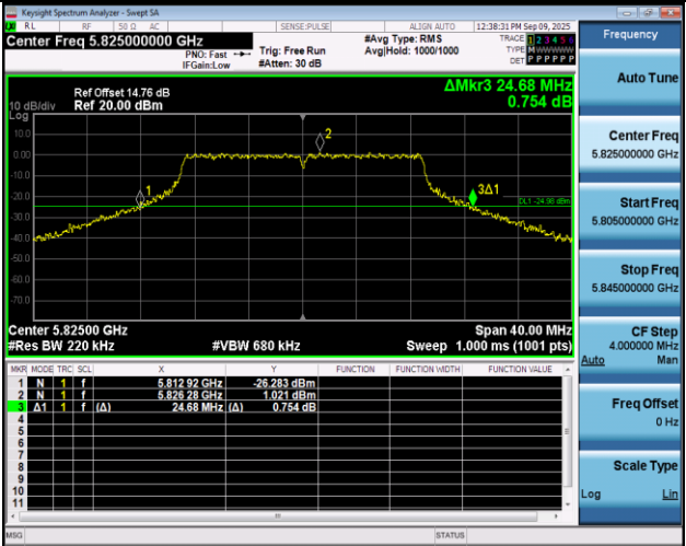
11N20SISO-Ant1-5825
