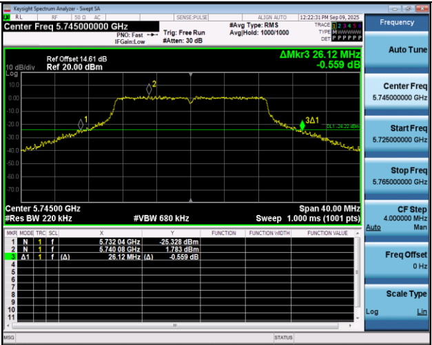
11N20SISO-Ant1-5745
