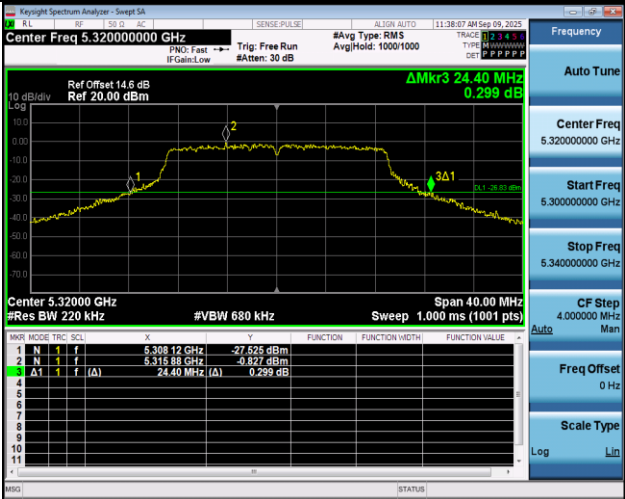
11N20SISO-Ant1-5320
