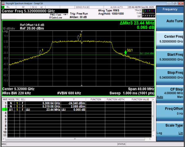
11A-Ant1-5320
