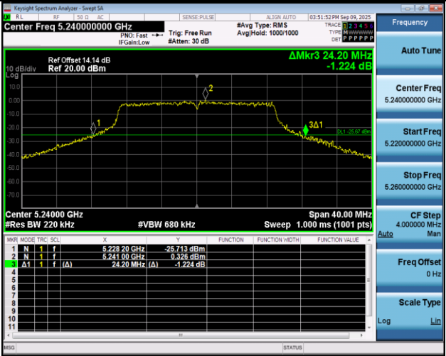
11AC20SISO-Ant1-5240
