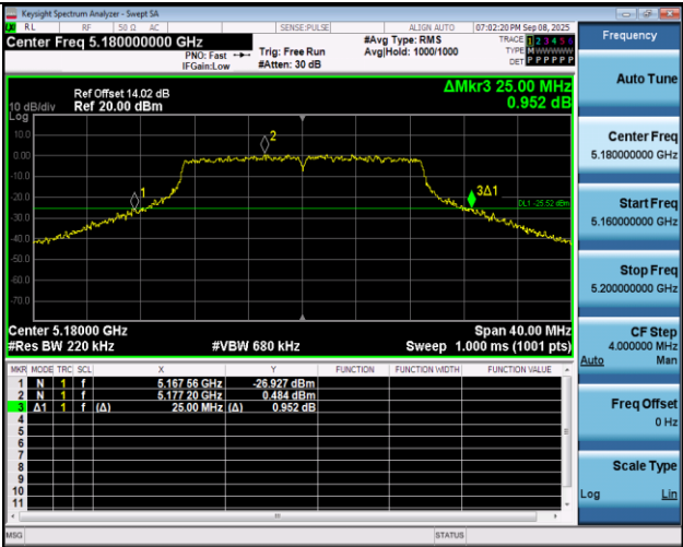
11N20SISO-Ant1-5180
