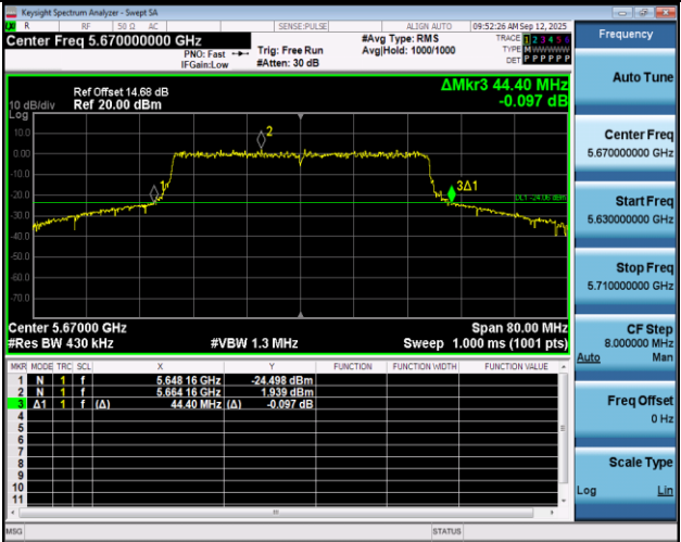
11AX40SISO-Ant1-5670
