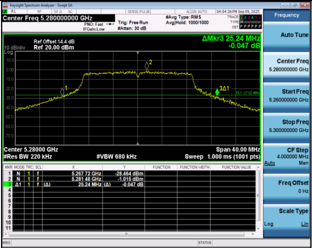
11AC20SISO-Ant1-5280
