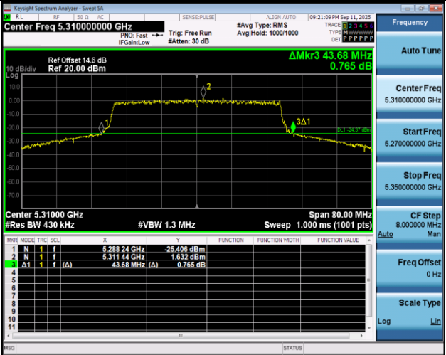
11AX40SISO-Ant1-5310
