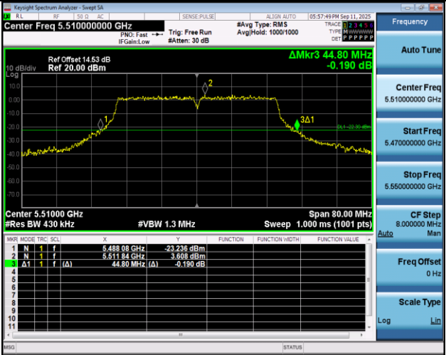
11AC40SISO-Ant1-5510
