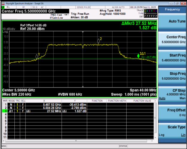
11AX20SISO-Ant1-5500
