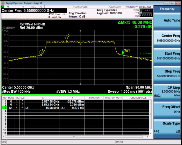
11AX40SISO-Ant1-5550
