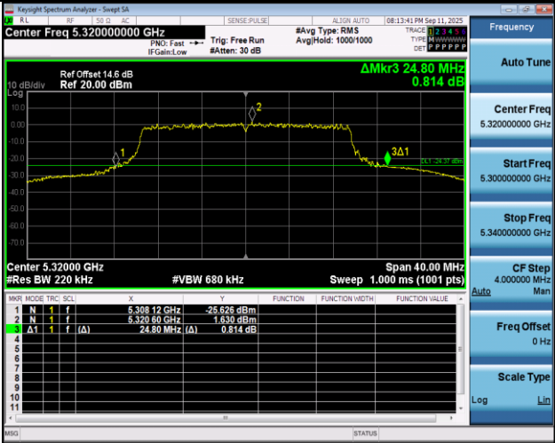
11AX20SISO-Ant1-5320
