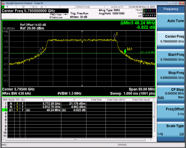
11AX40SISO-Ant1-5795
