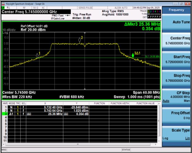
11AC20SISO-Ant1-5745
