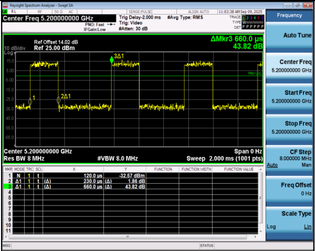
NTNV-11N20SISO-Ant1-5200
