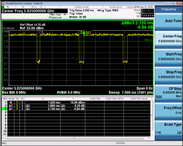
NTNV-11N20SISO-Ant1-5825
