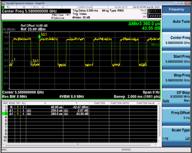
NTNV-11A-Ant1-5580
