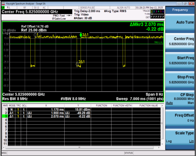
NTNV-11AC20SISO-Ant1-5825
