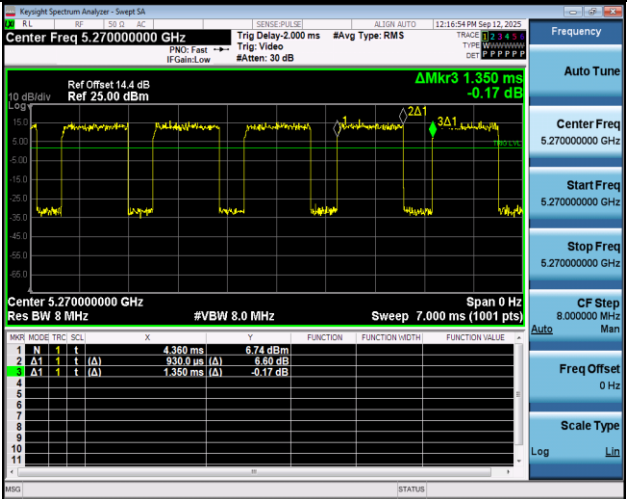
NTNV-11N40SISO-Ant1-5270
