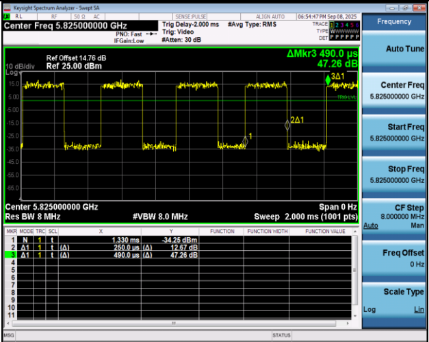
NTNV-11A-Ant1-5825
