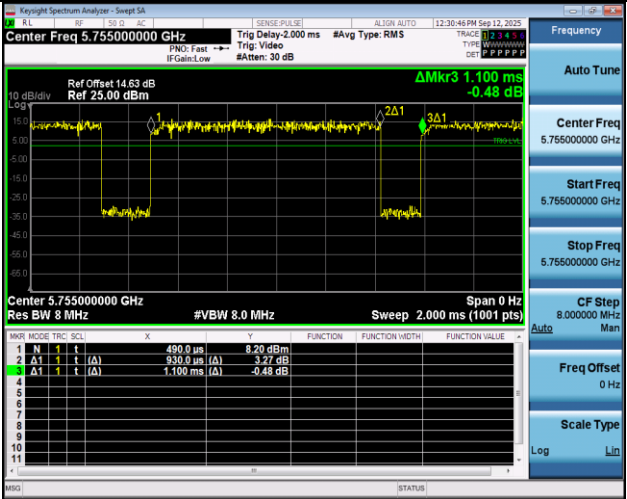
NTNV-11N40SISO-Ant1-5755
