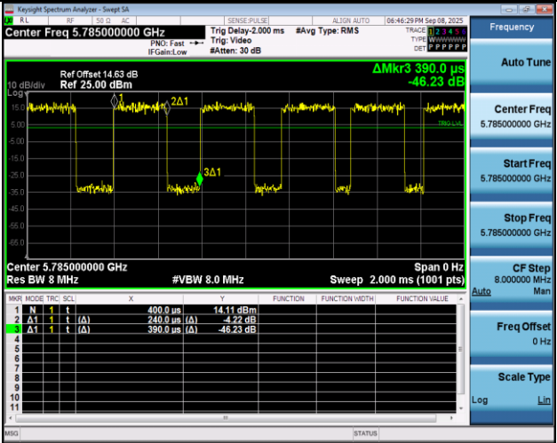
NTNV-11A-Ant1-5785
