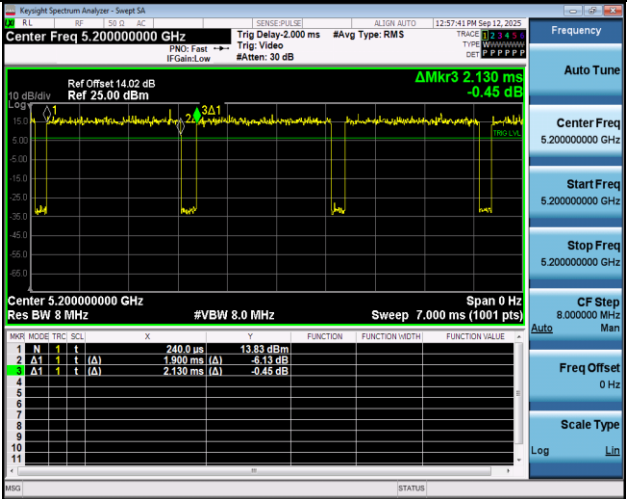
NTNV-11AC20SISO-Ant1-5200
