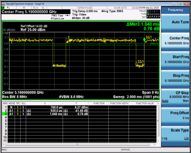
NTNV-11N40SISO-Ant1-5190
