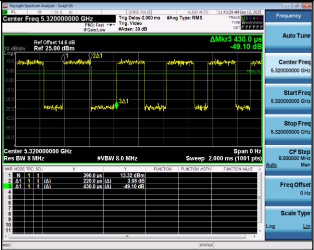
NTNV-11N20SISO-Ant1-5320
