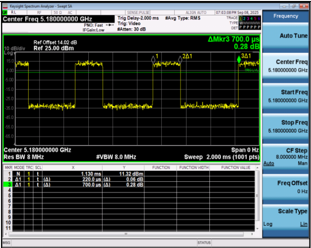
NTNV-11N20SISO-Ant1-5180
