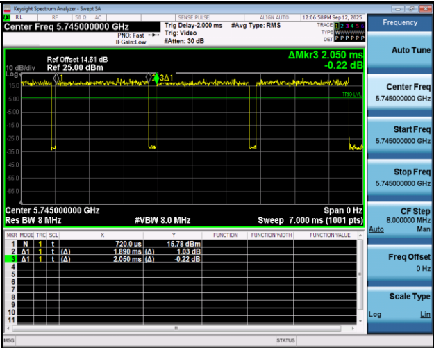
NTNV-11N20SISO-Ant1-5745
