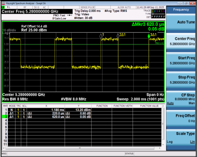
NTNV-11N20SISO-Ant1-5280
