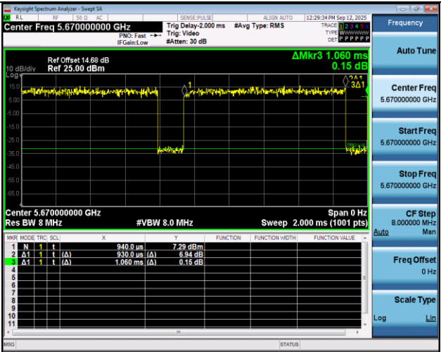
NTNV-11N40SISO-Ant1-5670
