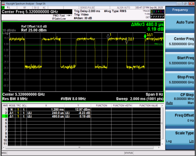
NTNV-11A-Ant1-5320
