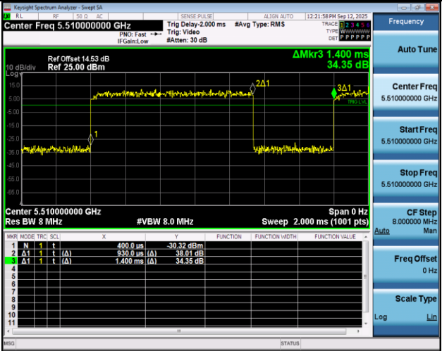
NTNV-11N40SISO-Ant1-5510
