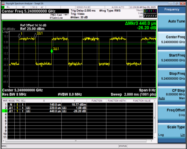
NTNV-11N20SISO-Ant1-5240
