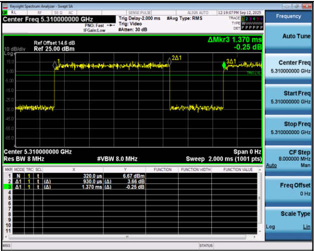
NTNV-11N40SISO-Ant1-5310
