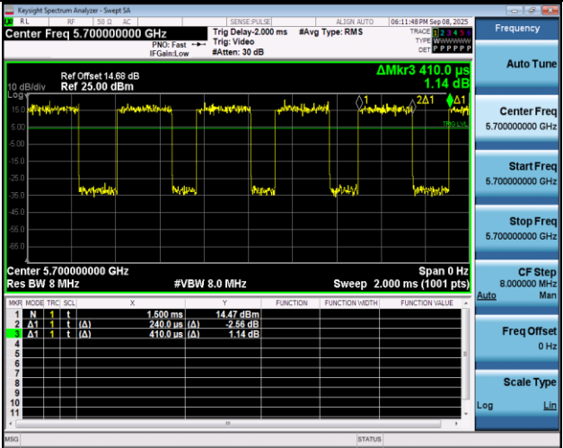
NTNV-11A-Ant1-5700
