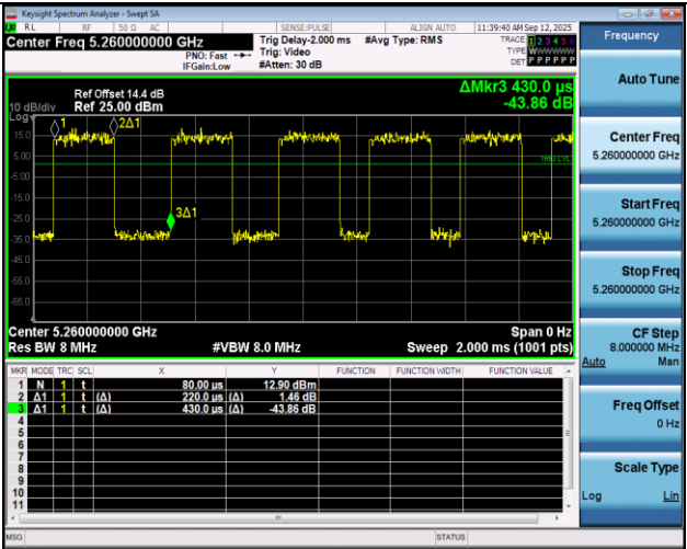
NTNV-11N20SISO-Ant1-5260
