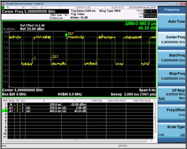
NTNV-11A-Ant1-5260
