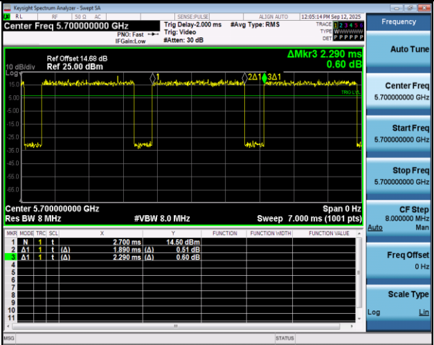
NTNV-11N20SISO-Ant1-5700
