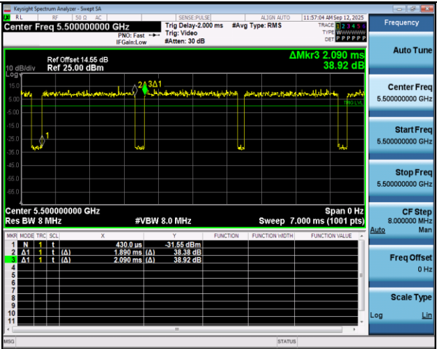
NTNV-11N20SISO-Ant1-5500
