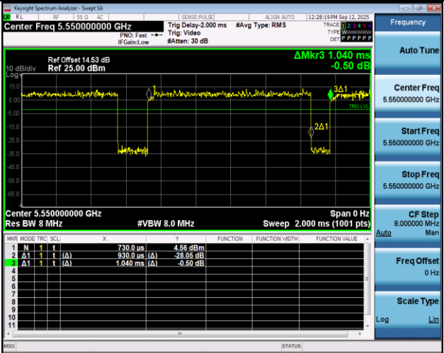
NTNV-11N40SISO-Ant1-5550
