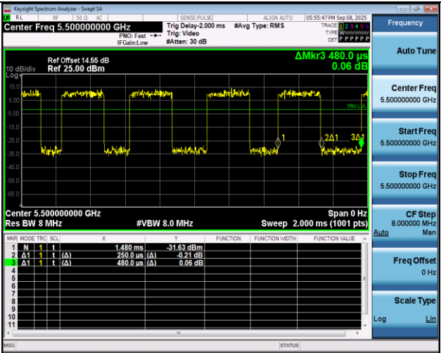
NTNV-11A-Ant1-5500
