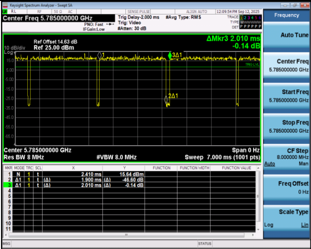
NTNV-11N20SISO-Ant1-5785
