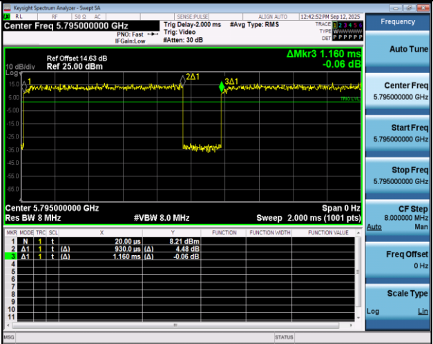
NTNV-11N40SISO-Ant1-5795
