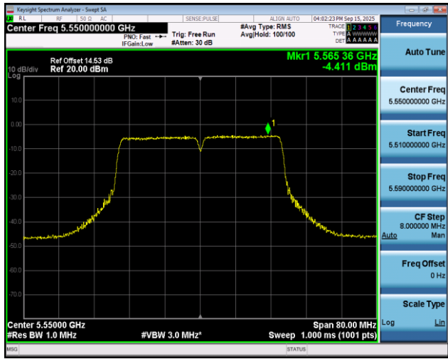
11AC40SISO-Ant1-5550-PASS
