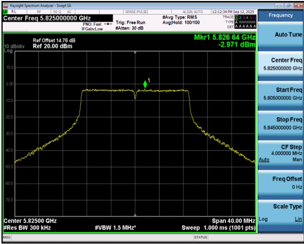
11N20SISO-Ant1-5825-PASS
