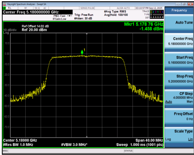
11AX20SISO-Ant1-5180-PASS
