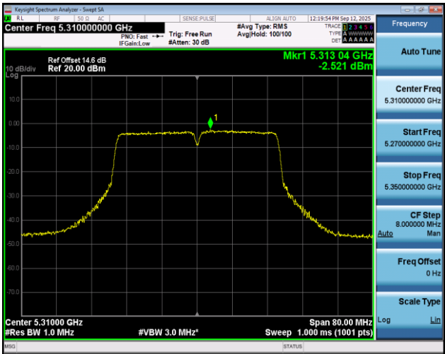
11N40SISO-Ant1-5310-PASS
