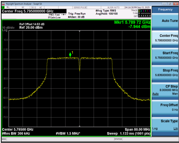
11AC40SISO-Ant1-5795-PASS
