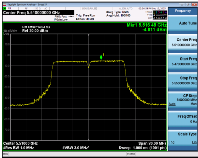
11AC40SISO-Ant1-5510-PASS
