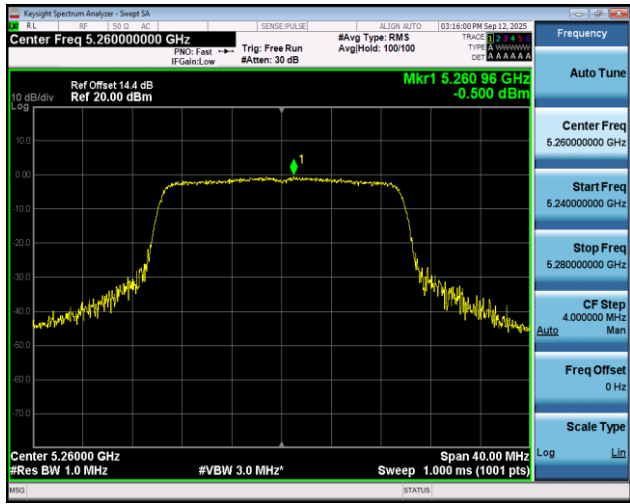
11AX20SISO-Ant1-5260-PASS
