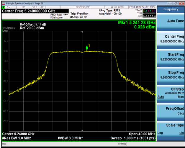
11AC20SISO-Ant1-5240-PASS
