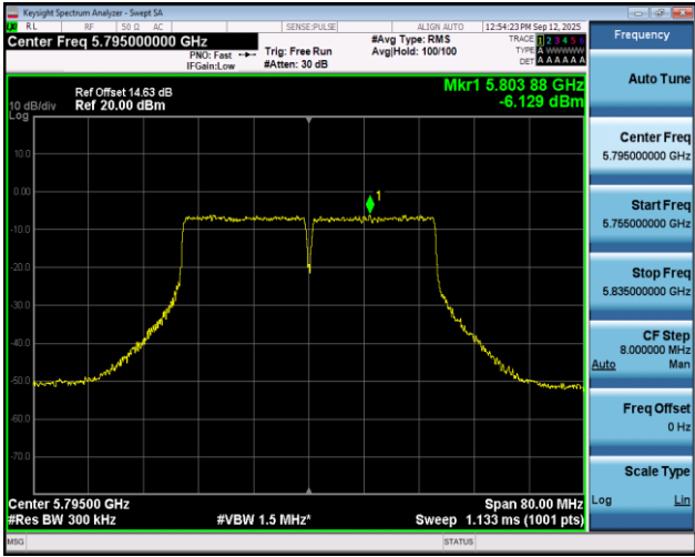
11N40SISO-Ant1-5795-PASS
