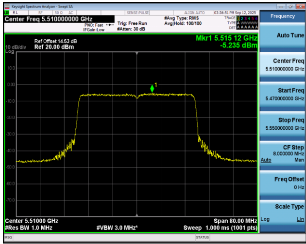
11AX40SISO-Ant1-5510-PASS
