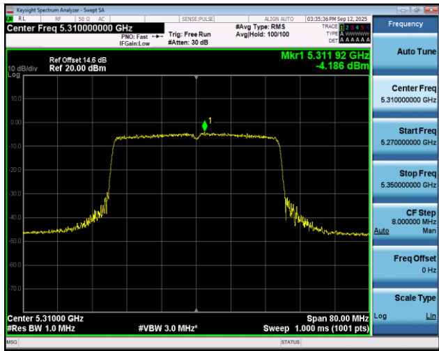
11AX40SISO-Ant1-5310-PASS
