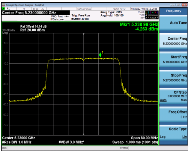
11AX40SISO-Ant1-5230-PASS
