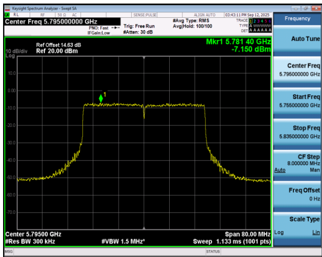
11AX40SISO-Ant1-5795-PASS
