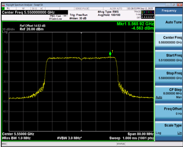
11AX40SISO-Ant1-5550-PASS
