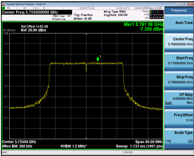
11AX40SISO-Ant1-5755-PASS
