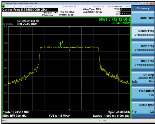
11AX20SISO-Ant1-5745-PASS
