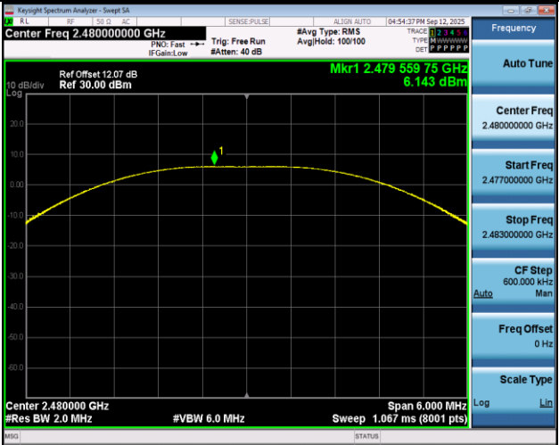
LE_2M-Ant1-2480-PASS
