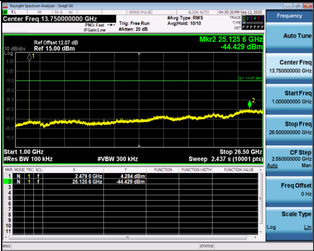
LE_1M-Ant1-2480-1000~26500-PASS
