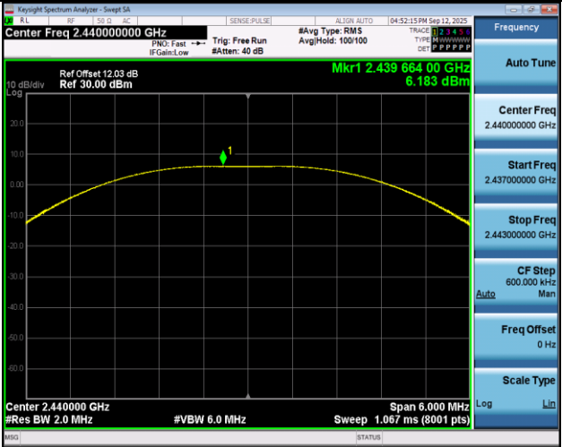
LE_2M-Ant1-2440-PASS
