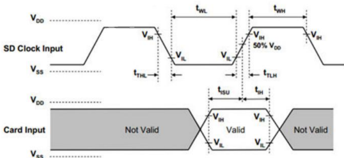
Figure 8-8 Input timing in HS mode
