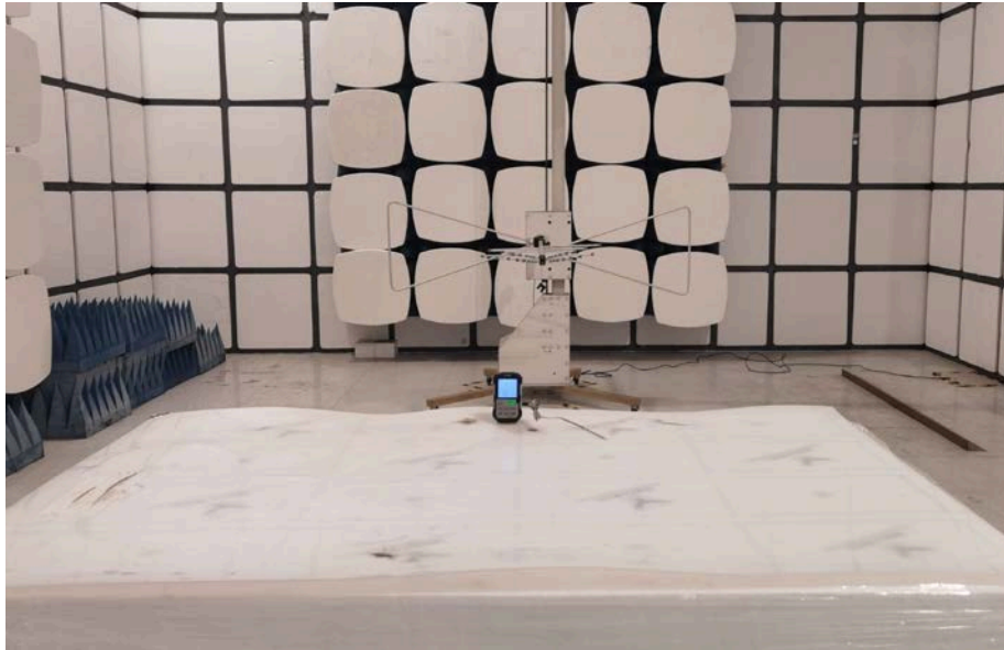
Spurious Emission Test Setup (Below 1GHz)
