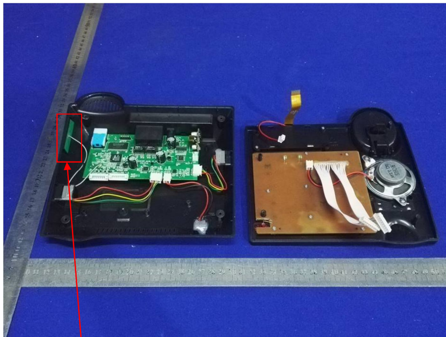
WIFI Antenna
