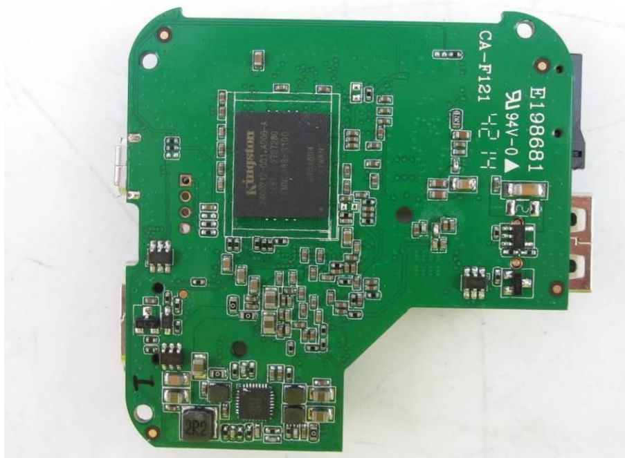
INTERNAL PHOTO OF SAMPLE - 4
