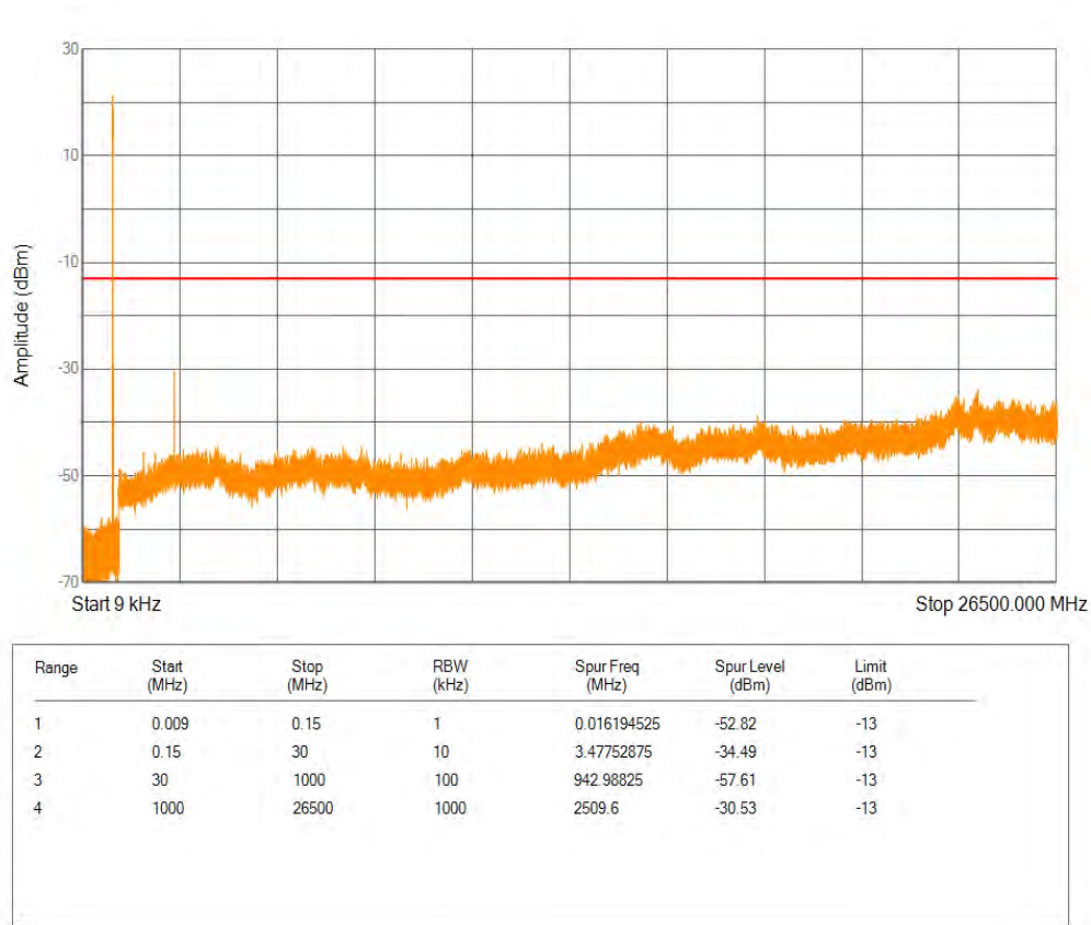
Band26(824-849) 16QAM BW=1.4MHz Channel=26915 RB Size=6 Position=#0
