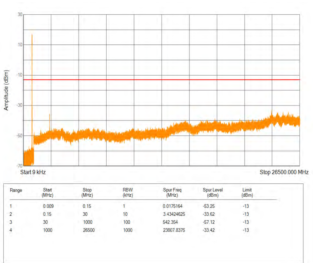
Band26(824-849) QPSK BW=3MHz Channel=26915 RB Size=15 Position=#0
