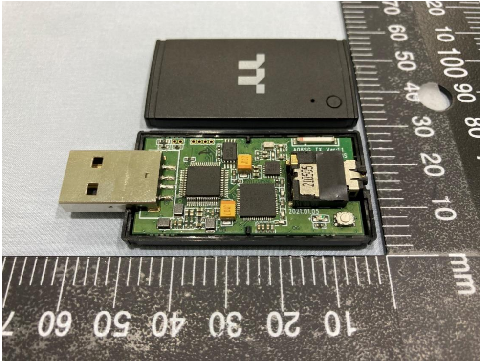
Internal Photos GHT-THF-RX Pic 1
