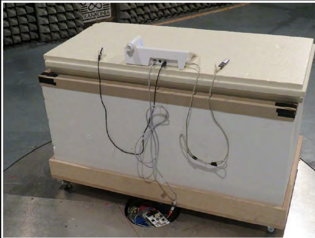
TEST SETUP - FOCUS - EUT CONFIGURATION 1
