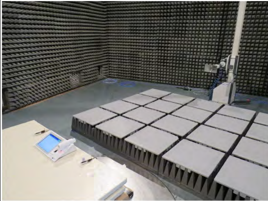
TEST SETUP - 1 GHz to 13 GHz - EUT CONFIGURATION 1
