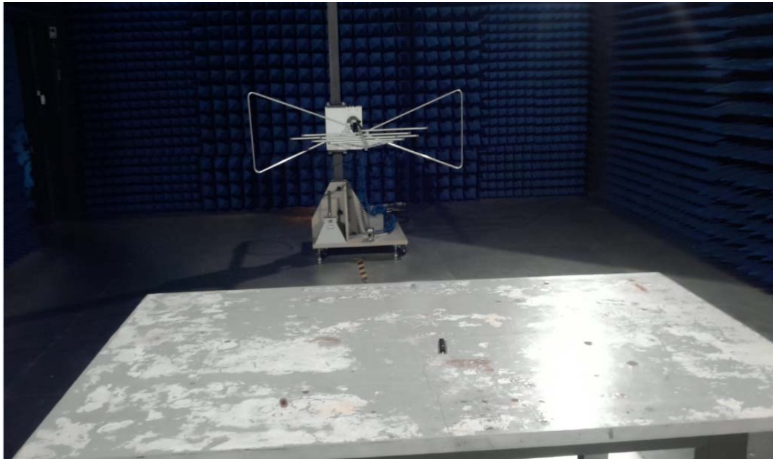
Radiated Emission test view
