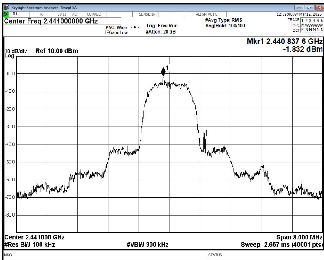
Tx. Spurious NVNT 3-DH5 2441MHz Ant0 Ref
