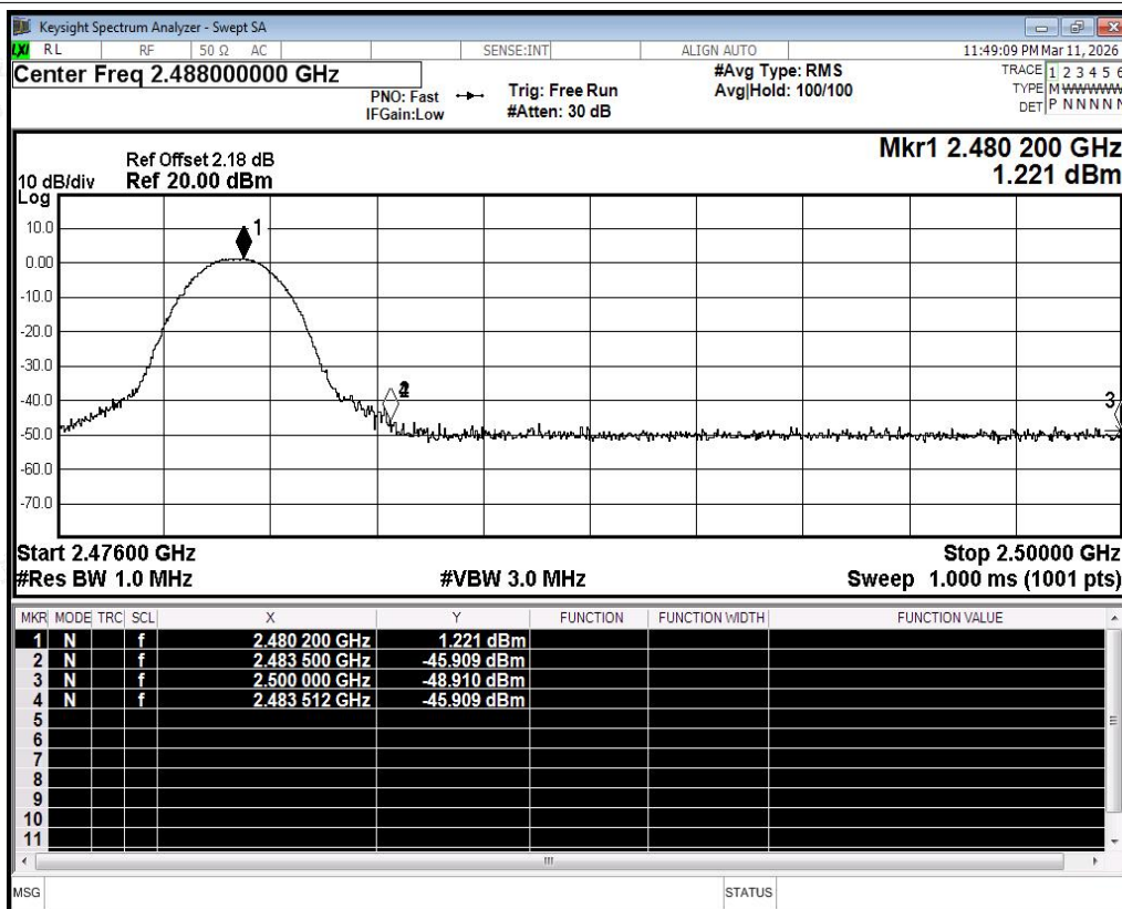
Restrict Band NVNT 2-DH5 2480MHz Ant0 No-Hopping Peak
