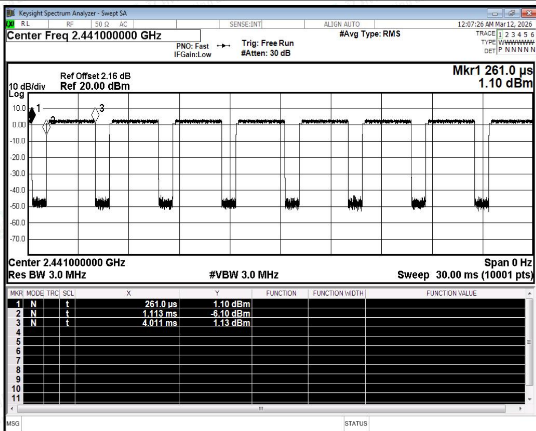
Duty Cycle NVNT 3-DH5 2441MHz Ant0
