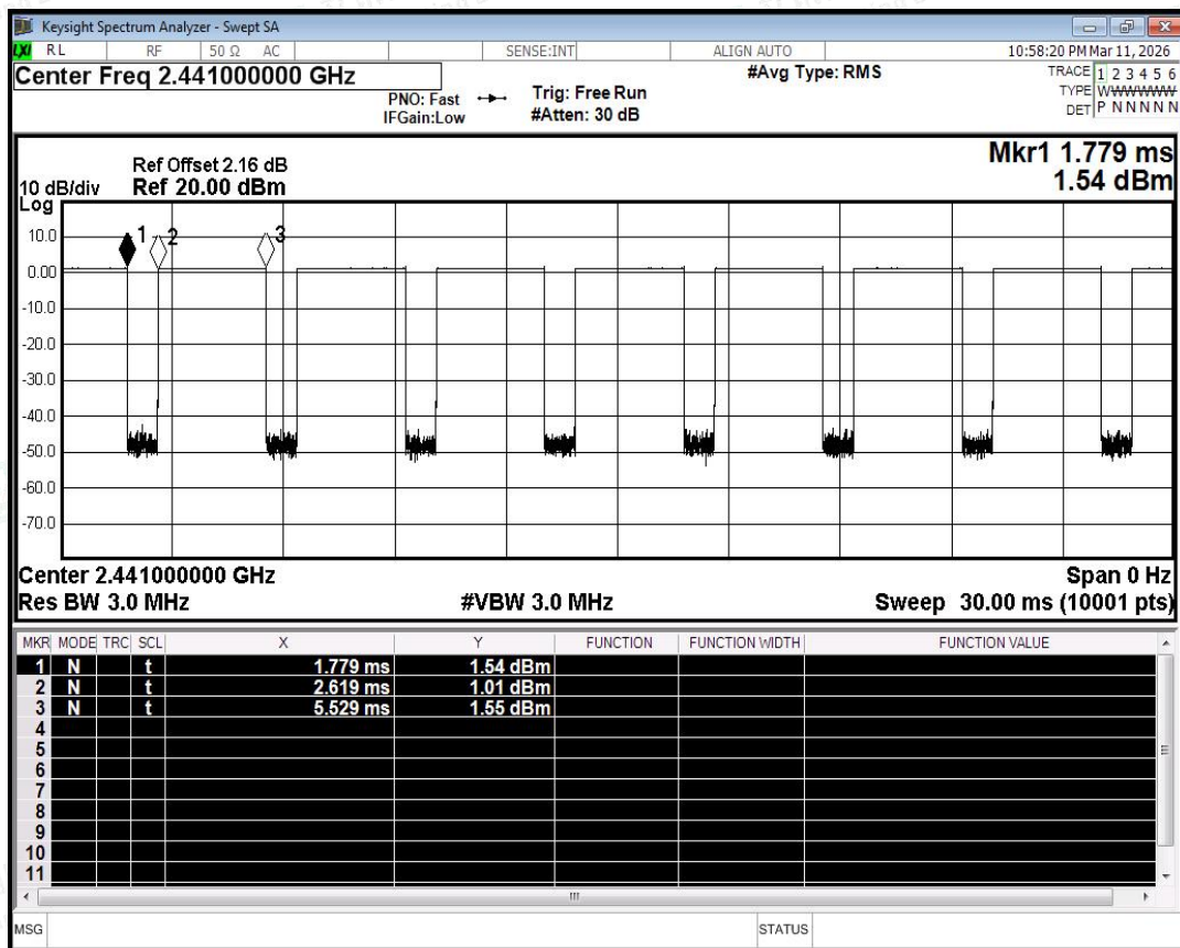
Duty Cycle NVNT 1-DH5 2441MHz Ant0
