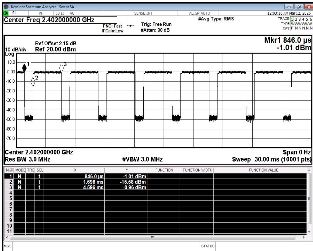
Duty Cycle NVNT 3-DH5 2402MHz Ant0
