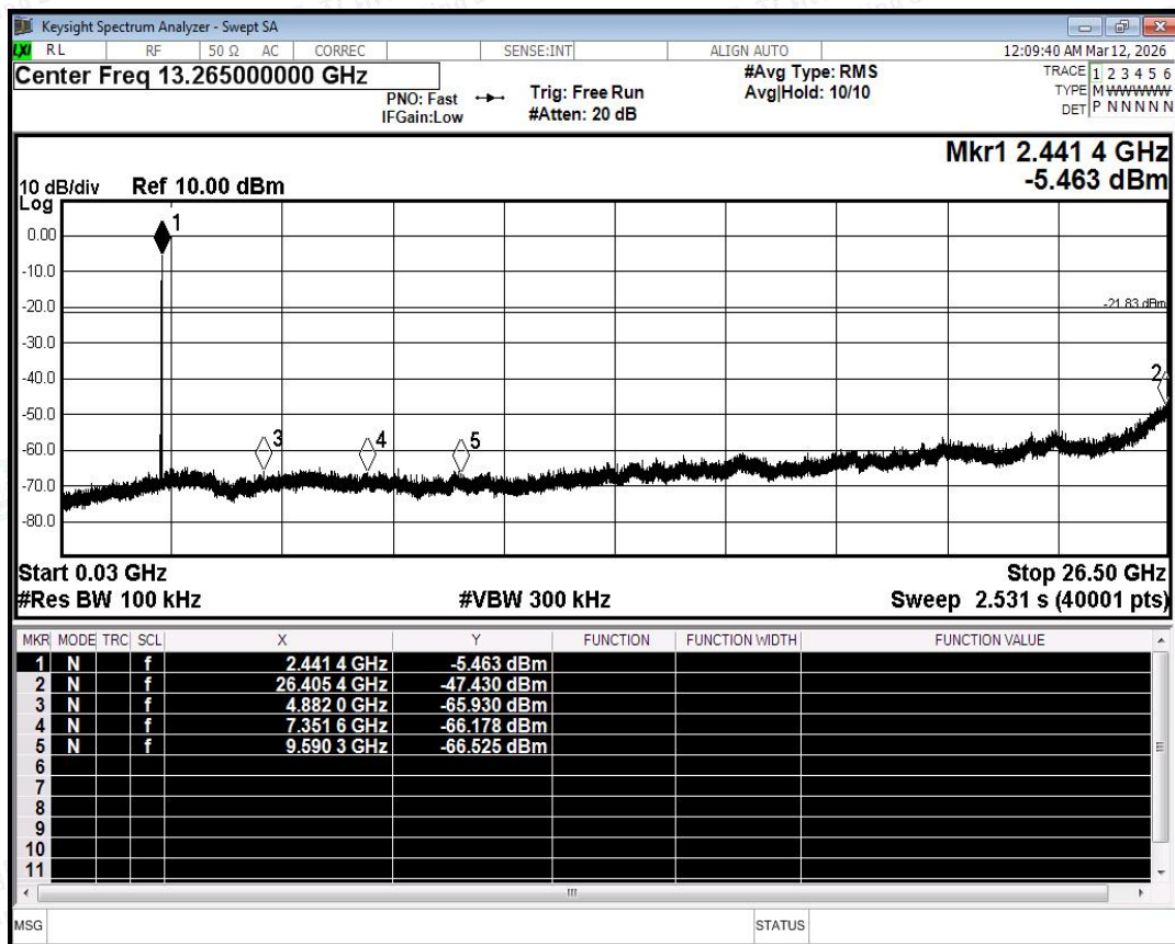
Tx. Spurious NVNT 3-DH5 2441MHz Ant0 Emission
