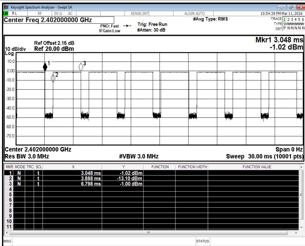
Duty Cycle NVNT 1-DH5 2402MHz Ant0
