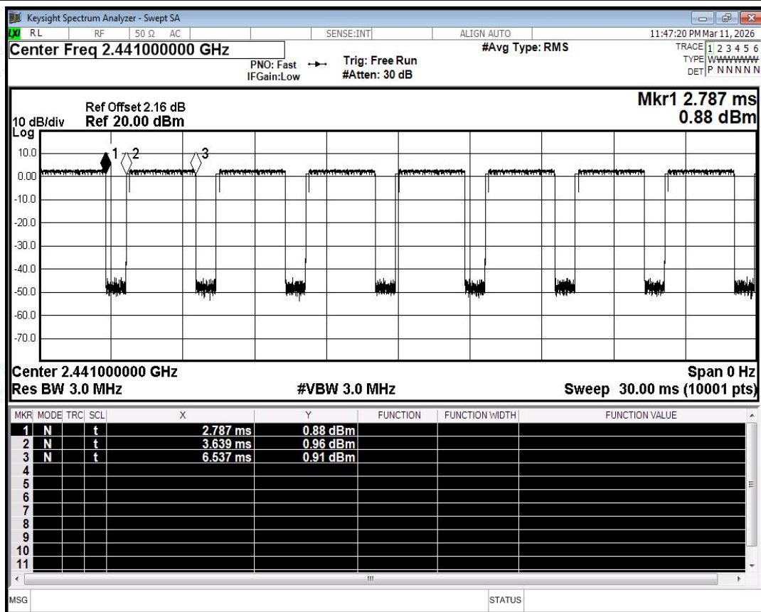
Duty Cycle NVNT 2-DH5 2441MHz Ant0
