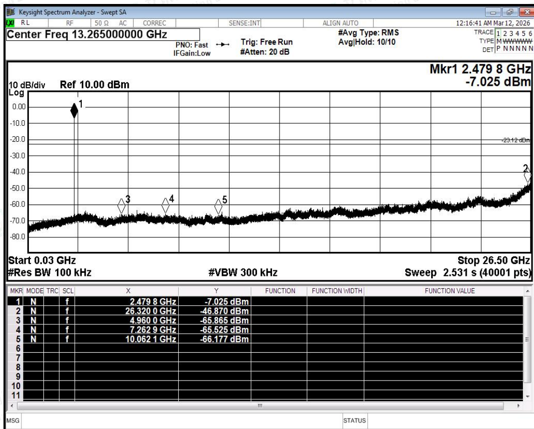
Tx. Spurious NVNT 3-DH5 2480MHz Ant0 Emission
