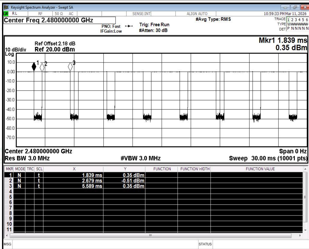
Duty Cycle NVNT 1-DH5 2480MHz Ant0
