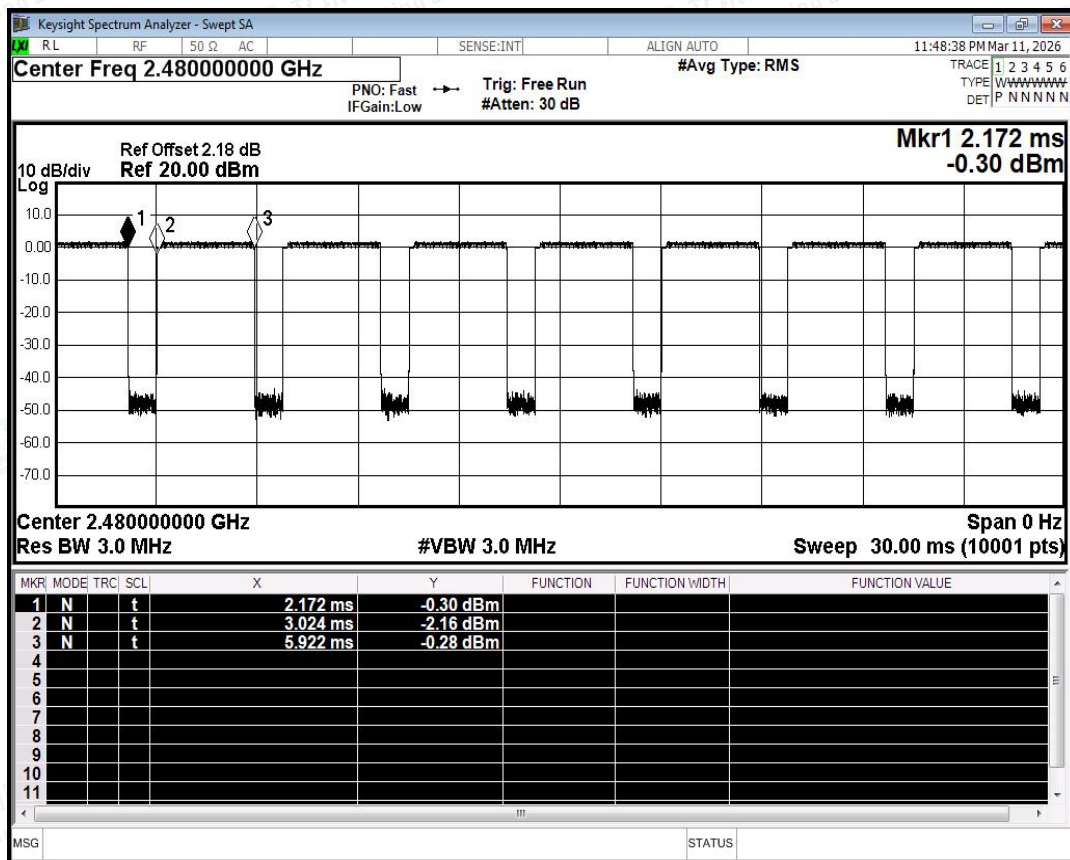
Duty Cycle NVNT 2-DH5 2480MHz Ant0
