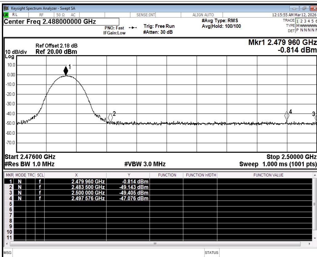
Restrict Band NVNT 3-DH5 2480MHz Ant0 No-Hopping Peak
