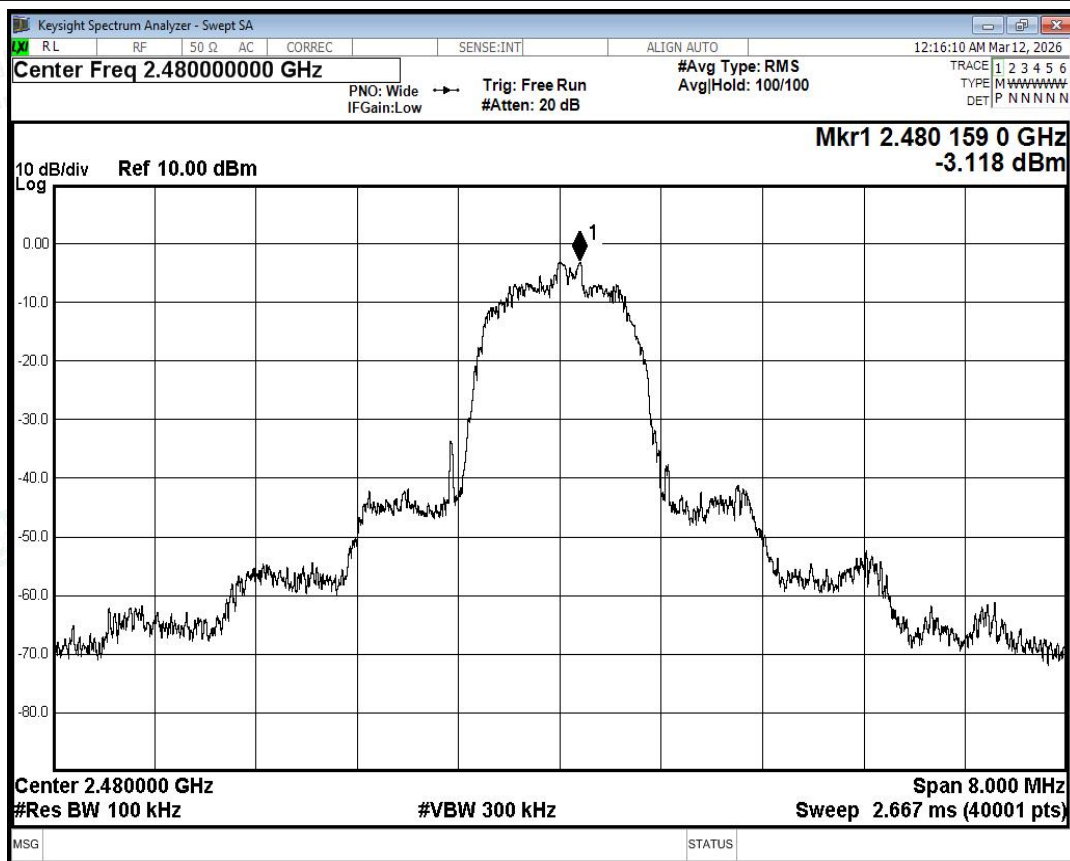
Tx. Spurious NVNT 3-DH5 2480MHz Ant0 Ref
