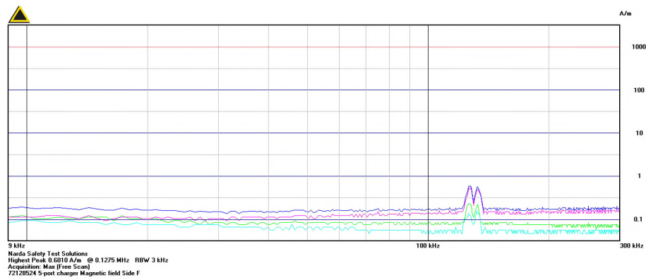
Graph 2.1.8.1-23 – H-Field Side F Plot 9kHz to 300kHz
