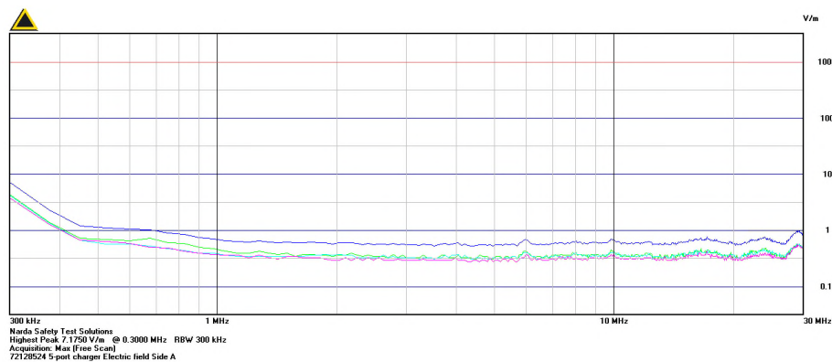
Graph 2.1.8.1-2 – E-Field Side A 300kHz to 30MHz
