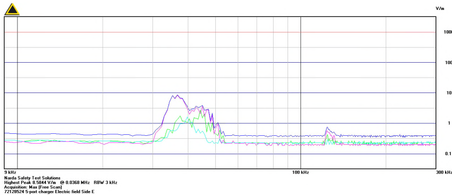
Graph 2.1.8.1-9 – E-Field Side E Plot 9kHz to 300kHz
