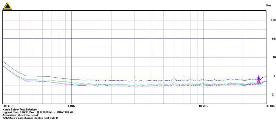
Graph 2.1.8.1-8 – E-Field Side D 300kHz to 30MHz
