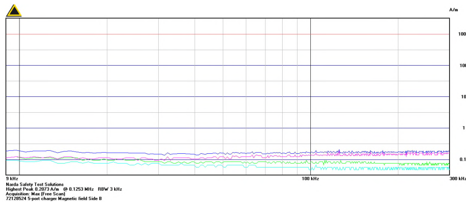
Graph 2.1.8.1-15 – H-Field Side B Plot 9kHz to 300kHz
