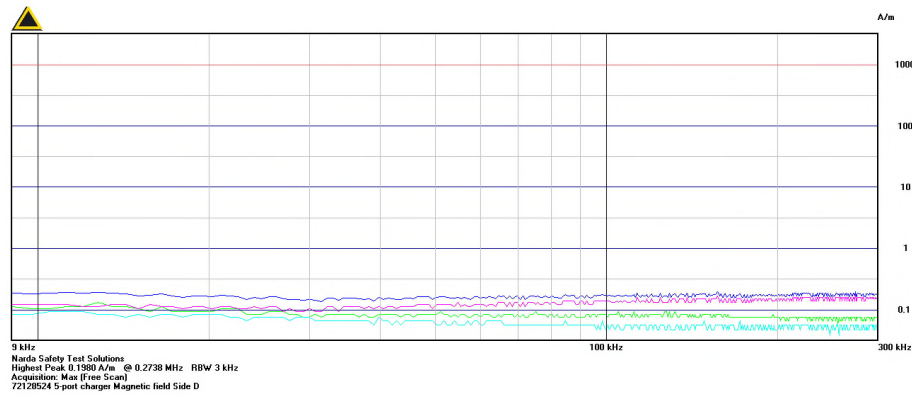
Graph 2.1.8.1-19 – H-Field Side D Plot 9kHz to 300kHz
