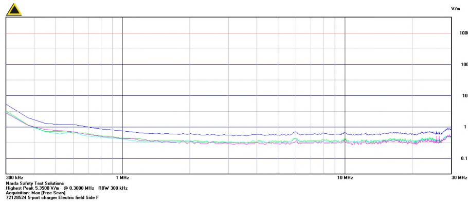
Graph 2.1.8.1-12 – E-Field Side F 300kHz to 30MHz
