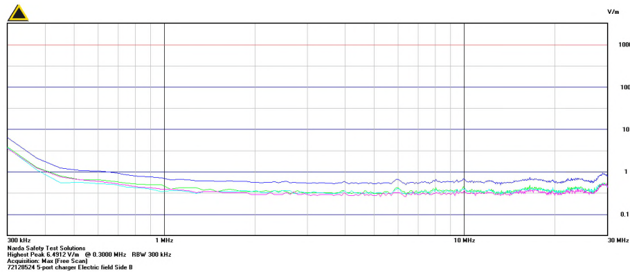
Graph 2.1.8.1-4 – E-Field Side B 300kHz to 30MHz
