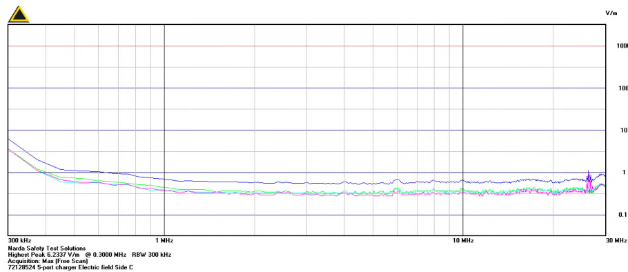
Graph 2.1.8.1-6 – E-Field Side C 300kHz to 30MHz
