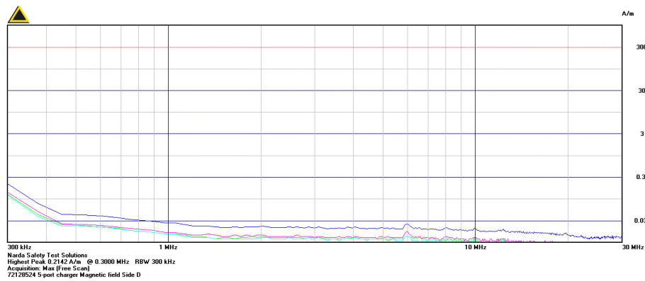
Graph 2.1.8.1-20 – H-Field Side D 300kHz to 30MHz
