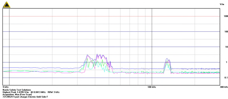
Graph 2.1.8.1-11 – E-Field Side F Plot 9kHz to 300kHz
