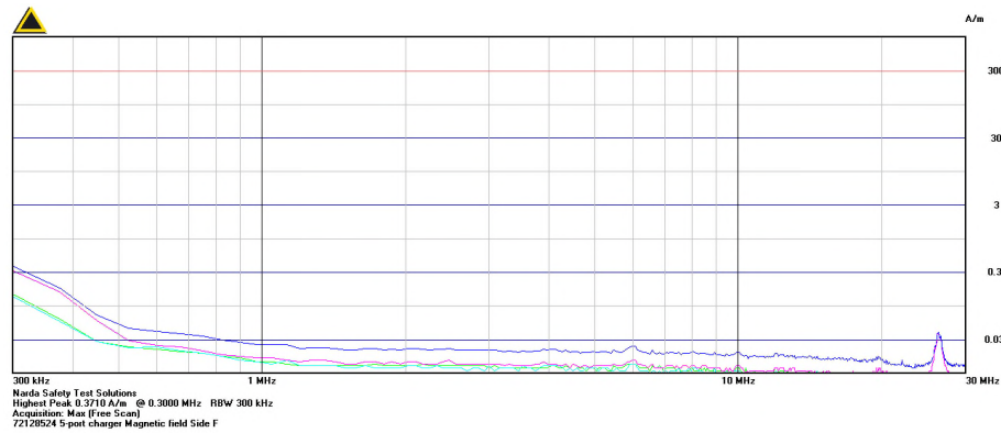
Graph 2.1.8.1-24 – H-Field Side F 300kHz to 30MHz
