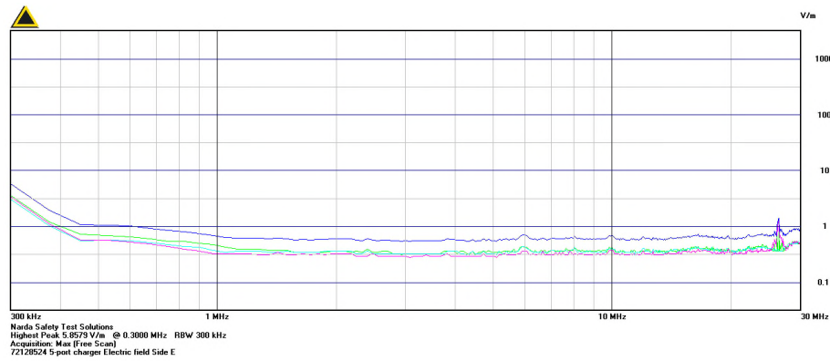
Graph 2.1.8.1-10 – E-Field SideE 300kHz to 30MHz
