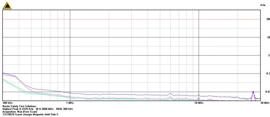
Graph 2.1.8.1-18 – H-Field Side C 300kHz to 30MHz
