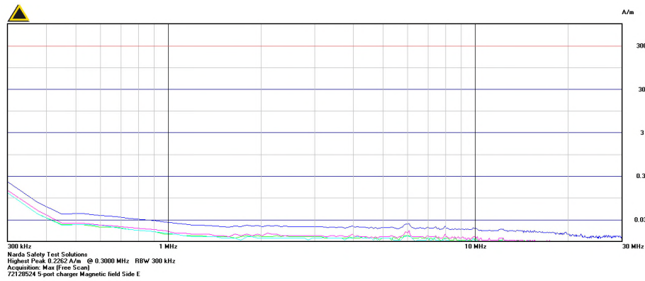
Graph 2.1.8.1-22 – H-Field SideE 300kHz to 30MHz
