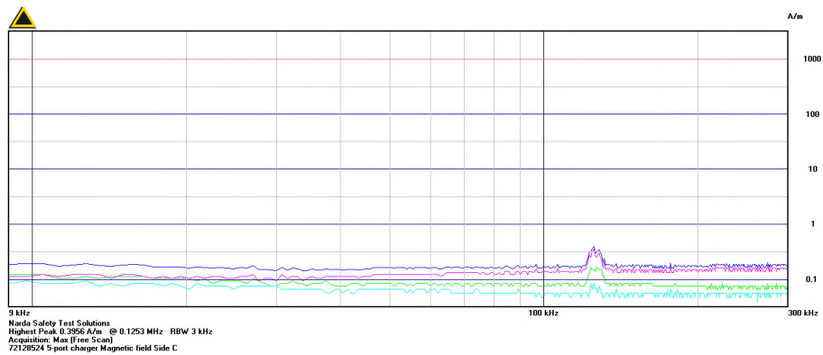
Graph 2.1.8.1-17 – H-Field Side C Plot 9kHz to 300kHz
