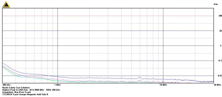
Graph 2.1.8.1-16 – H-Field Side B 300kHz to 30MHz
