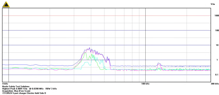
Graph 2.1.8.1-7 – E-Field Side D Plot 9kHz to 300kHz
