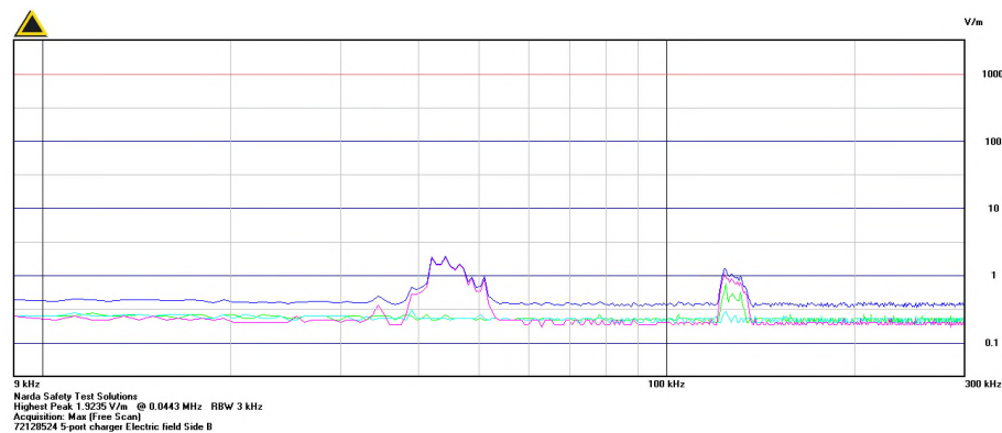
Graph 2.1.8.1-3 – E-Field Side B Plot 9kHz to 300kHz
