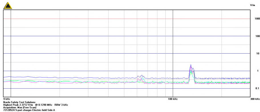
Graph 2.1.8.1-1 – E-Field Side A Plot 9kHz to 300kHz
