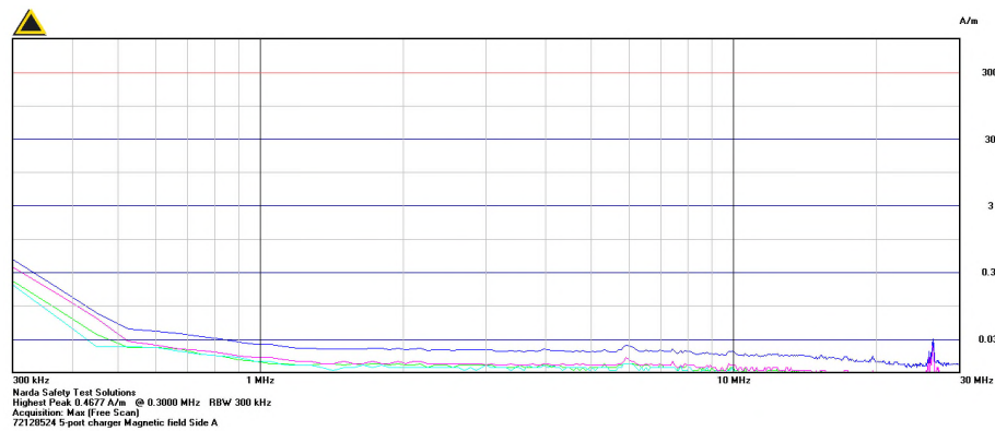
Graph 2.1.8.1-14 – H-Field Side A 300kHz to 30MHz
