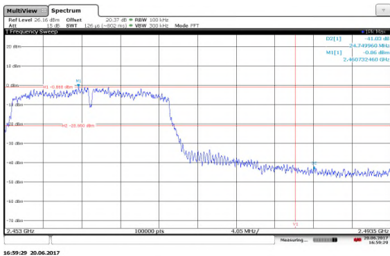
Figure 7.5.1.2-10: Upper Band-edge - 802.11g - 2462 MHz
