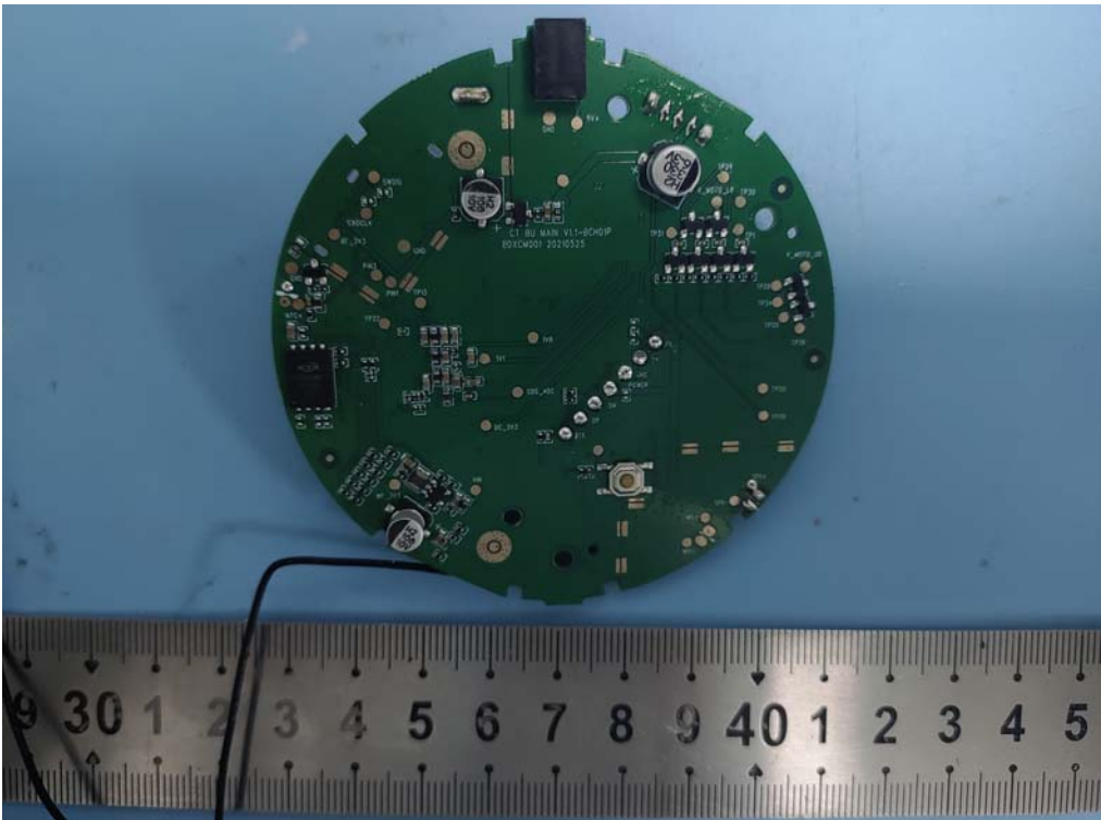
2.4G FHSS Antenna
