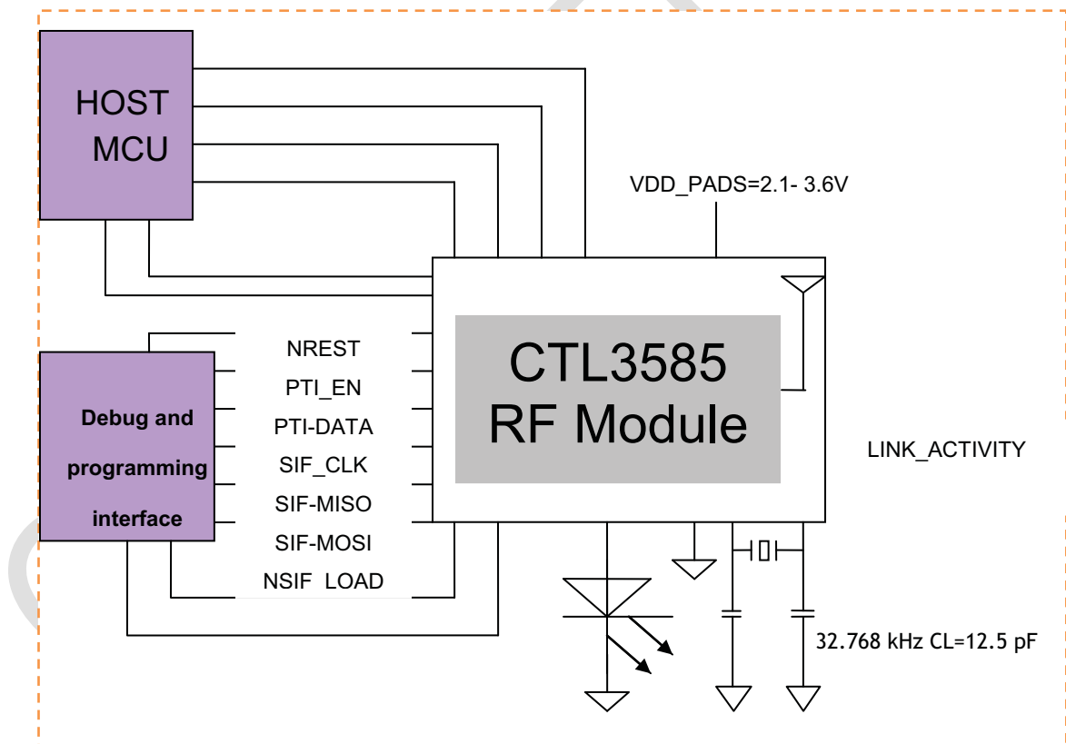
Figure 1: Example of application circuit
