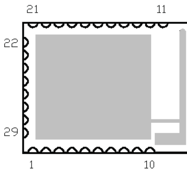
Figure 2: CTLA357/CTLB357 pin assignment
