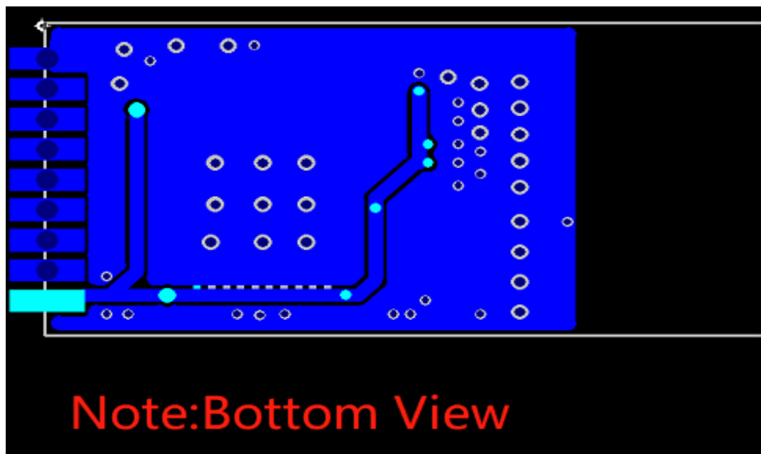
FIGURE 9 BOTTOM COPPER
