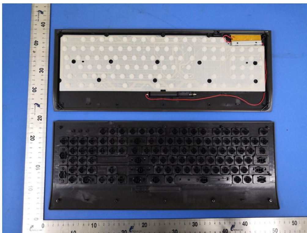
View of Product-5(model : KG9160)
