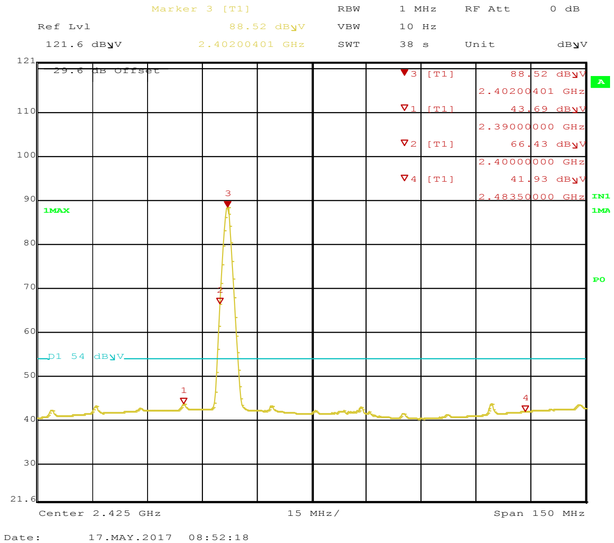
Figure 22: Radiated Emission at the Edge for Channel 2402 MHz at DH5 – Vertical (avg)
