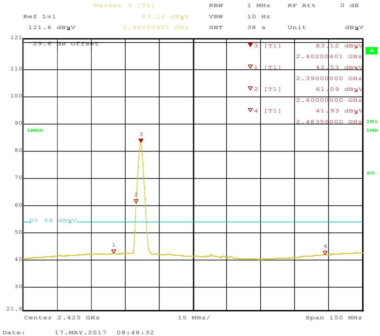
Figure 20: Radiated Emission at the Edge for Channel 2402 MHz at DH5 – Horizontal (Avg)
