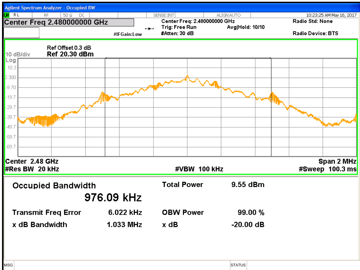
Figure 6: Occupied Bandwidth at 2480 MHz (DH5)
