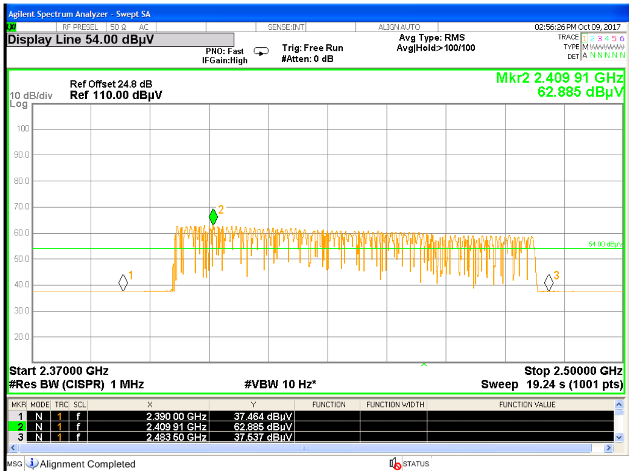
Figure 28: Radiated Emission at the Restricted Band Edge for Hopping Mode at DH5 – Horz. (Ave)
