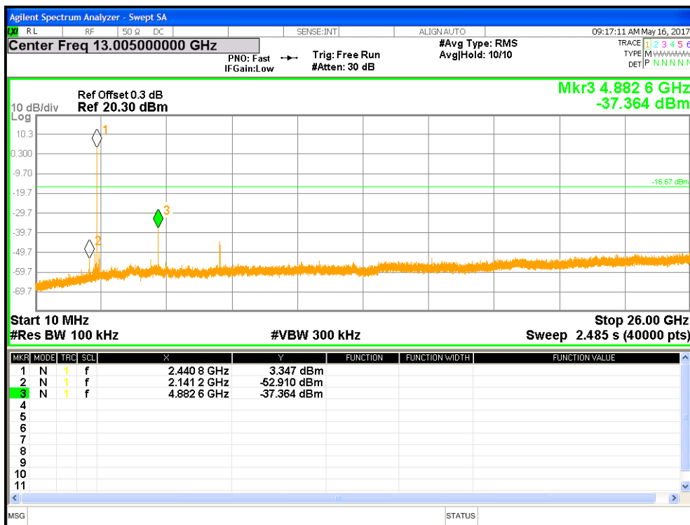
Figure 16: Out of Band Emission Requirements at 2442 MHz – DH1
