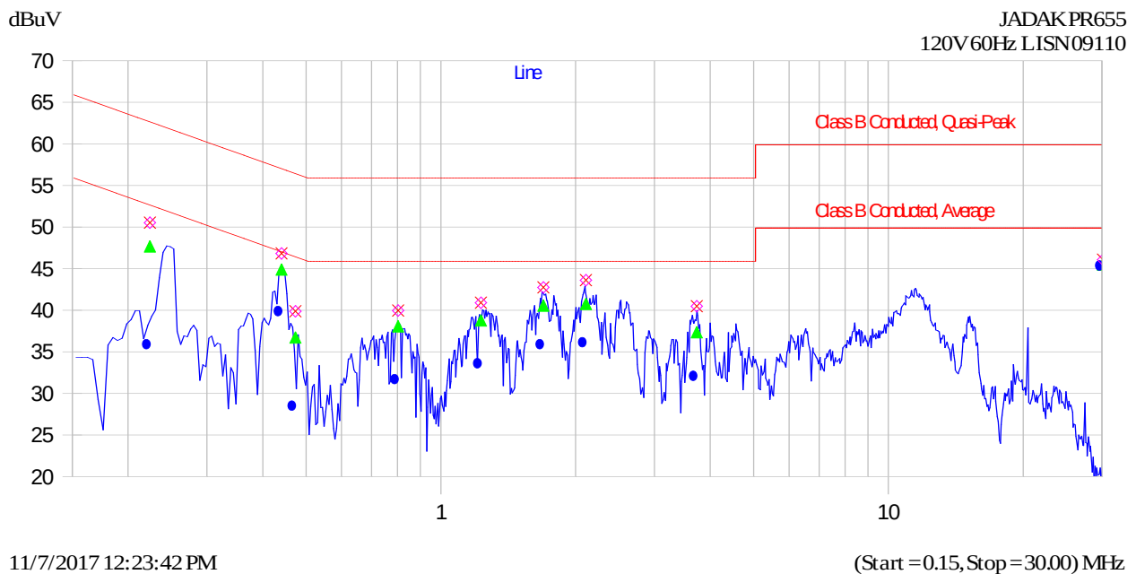
150kHz to 30 MHz Plot for Line 1 (Hot)
