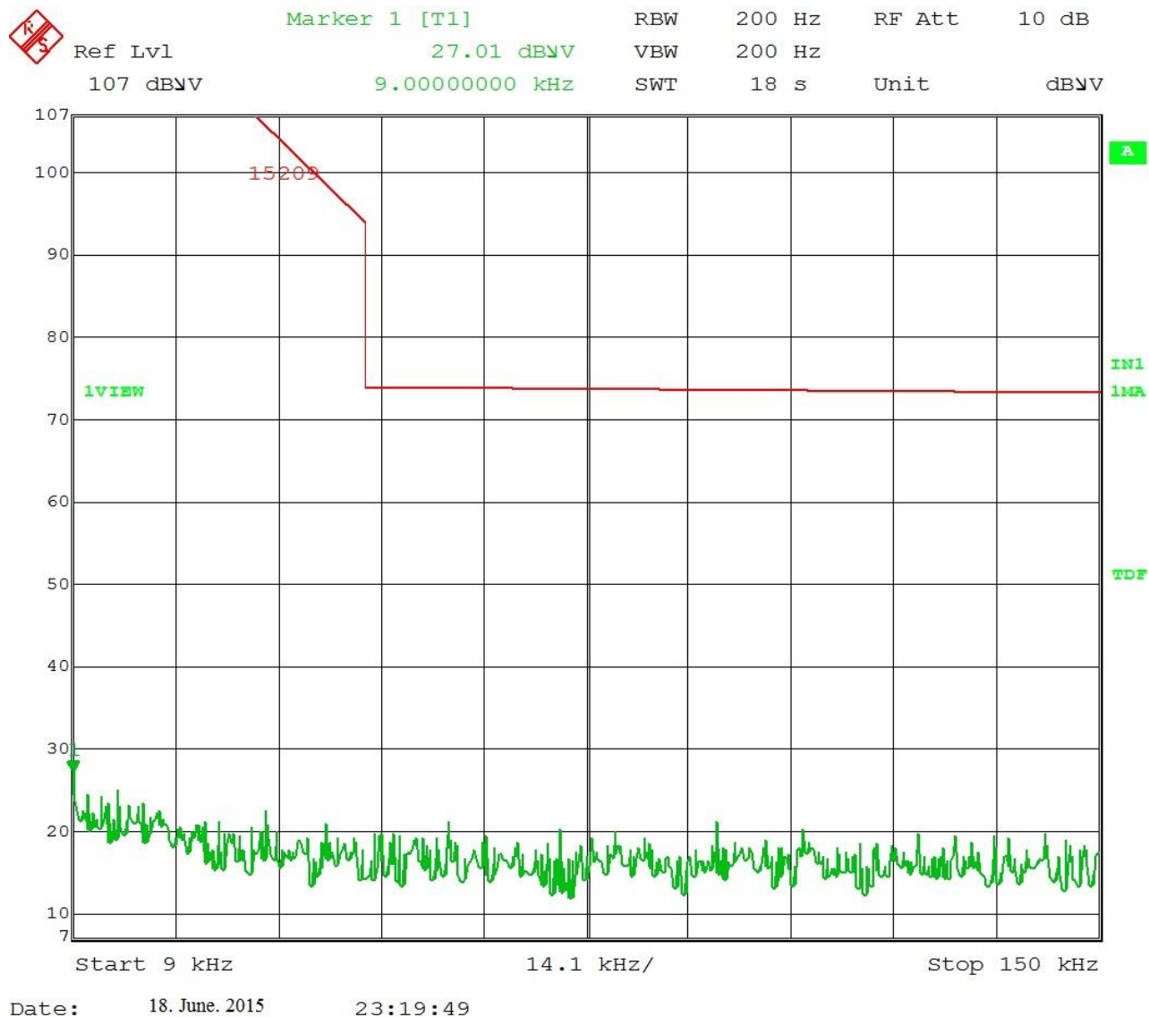
Figure 5 – Spurious Emissions (Perpendicular) 9 kHz to 150 kHz Measured at 1m distance
