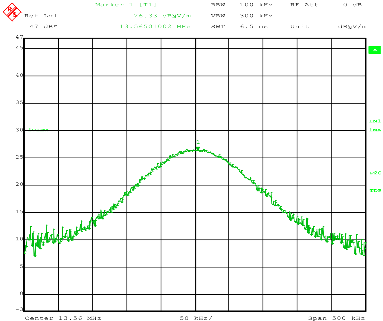
Figure 1 – Peak Field Strength Parallel Polarity is 26.33 dBuV at 1m
