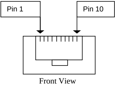
RJ45 Pin Definition and Function
