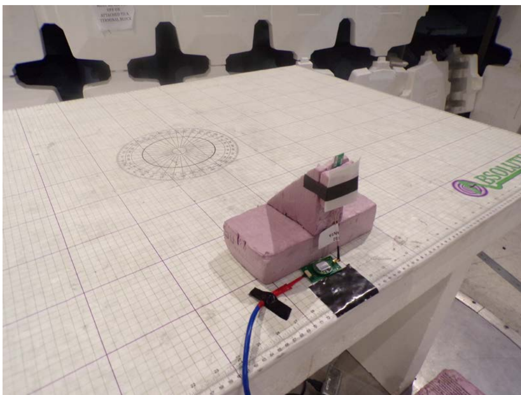
30MHz-1GHz Close-up
