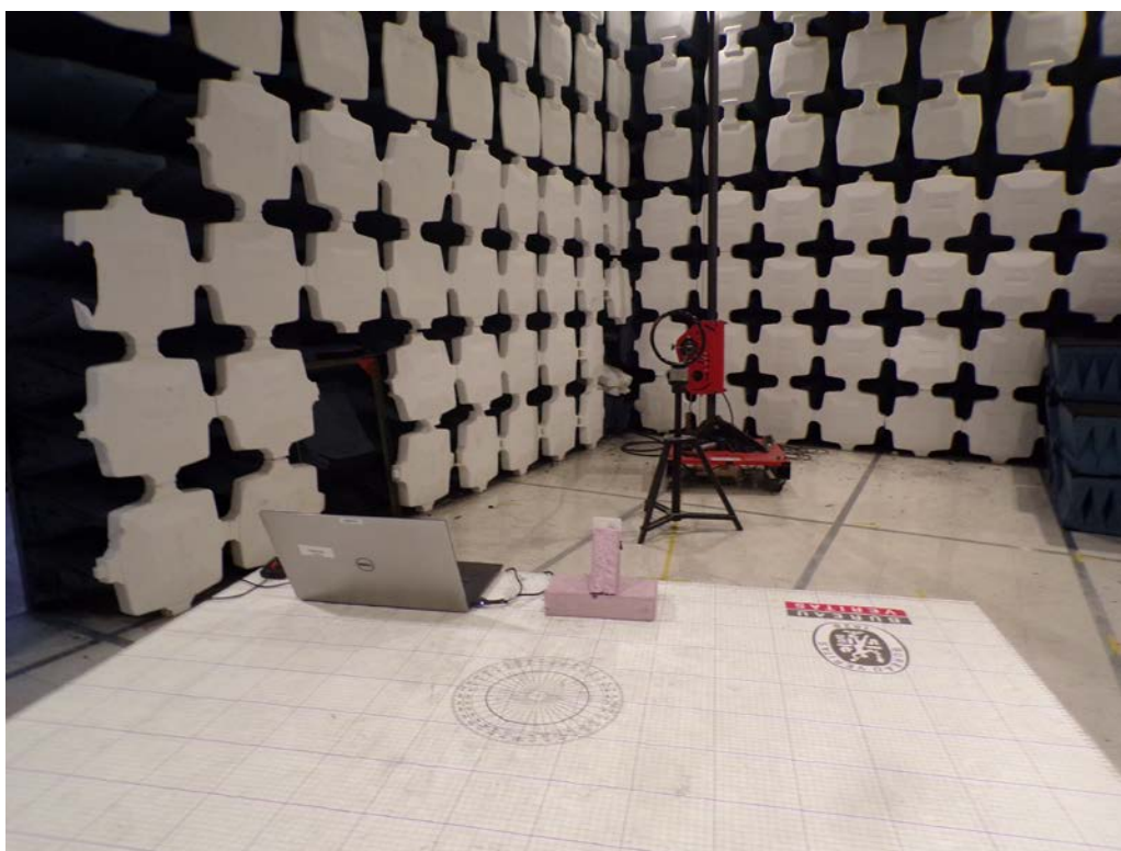
1-30MHz Parallel
