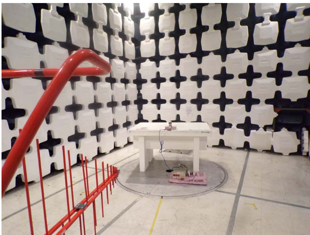
30MHz-1GHz Front
