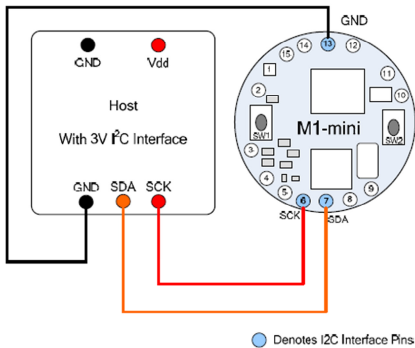
Figure 8: I2C Connection: M1-Mini to Host
