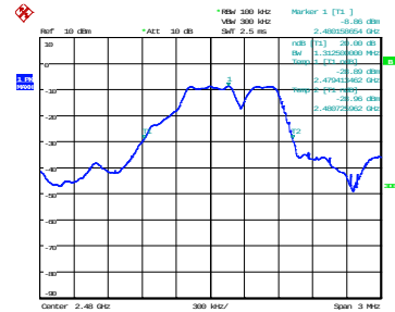
1 Mbps - 2480 MHz
