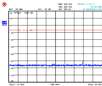
13 GHz – 18 GHz
