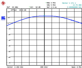
1 Mbps - 2402 MHz
