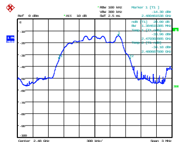
3 Mbps - 2480 MHz
