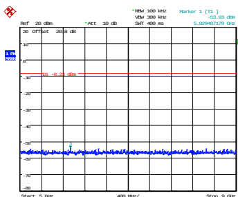
5 GHz – 9 GHz
