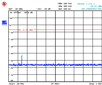
30 MHz – 1 GHz
