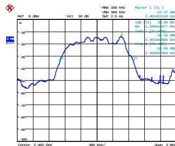
3 Mbps - 2402 MHz
