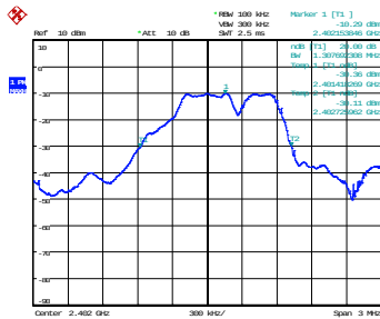
1 Mbps - 2402 MHz
