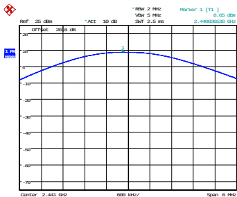
2 Mbps - 2441 MHz
