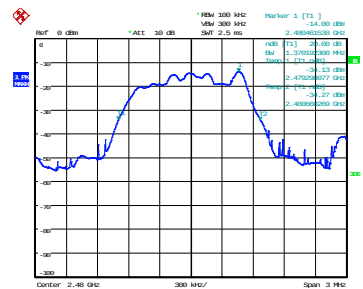
2 Mbps - 2480 MHz
