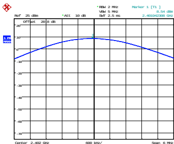
3 Mbps - 2402 MHz
