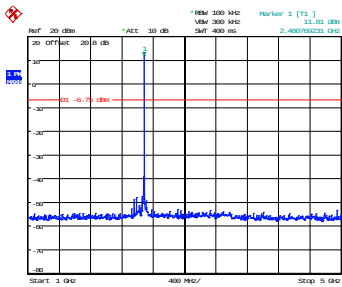
1 GHz – 5 GHz
