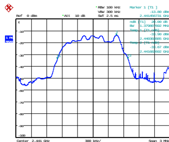
3 Mbps - 2441 MHz
