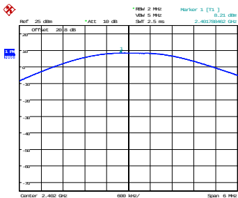
2 Mbps - 2402 MHz
