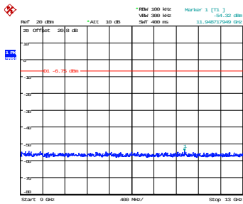
9 GHz – 13 GHz
