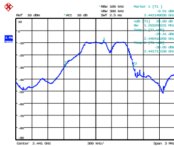
1 Mbps - 2441 MHz
