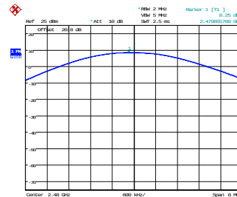
2 Mbps - 2480 MHz
