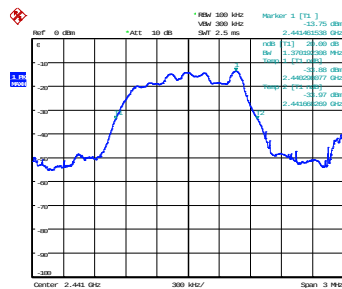
2 Mbps - 2441 MHz
