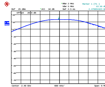
1 Mbps - 2480 MHz
