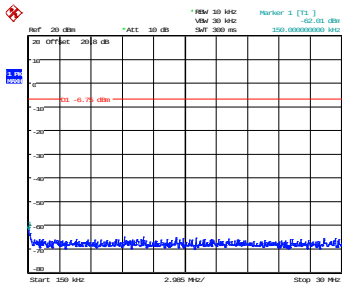
150 kHz – 30 MHz
