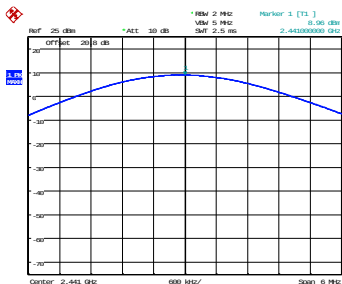
3 Mbps - 2441 MHz
