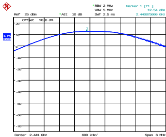
1 Mbps - 2441 MHz
