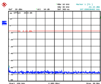
150 kHz – 30 MHz
