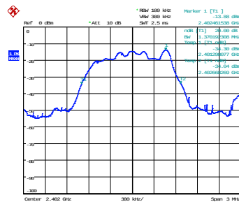
2 Mbps - 2402 MHz
