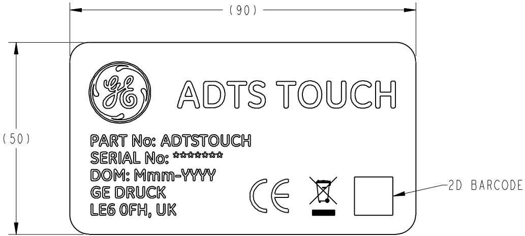
PRODUCT LABEL, ITEM 2 MARKING DETAILS AS SHOWN FONT: GE INSPIRA BOLD
