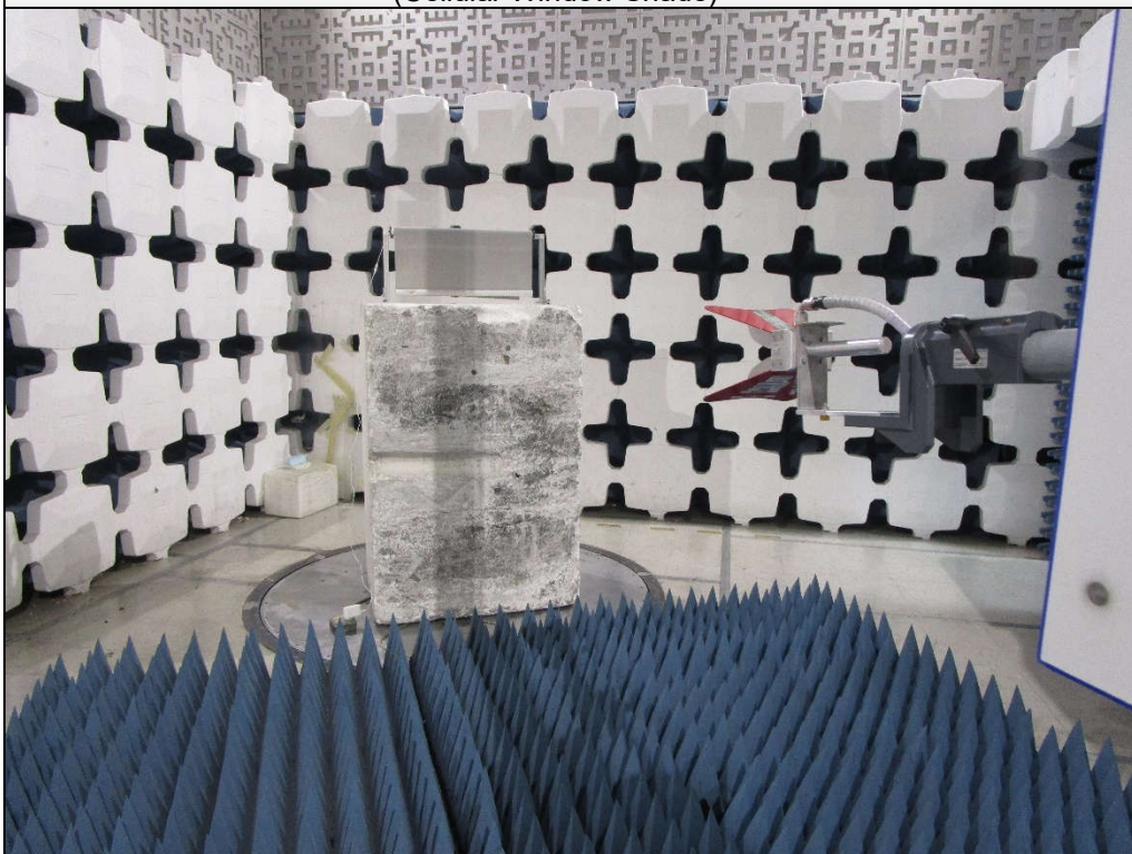
Test Setup for Spurious Emissions: Above 1GHz, Vertical Polarization (Cellular Window Shade)
